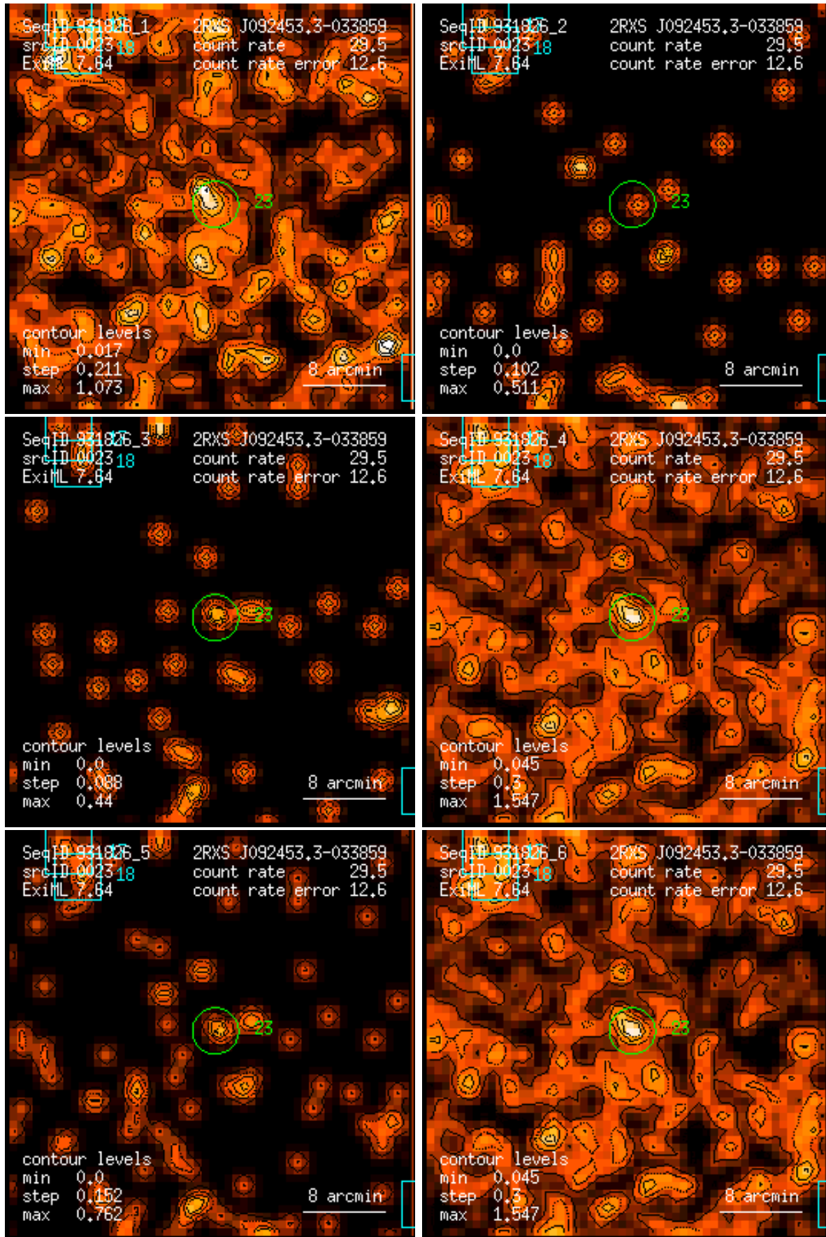
Figure 23: RASS 931826: detection 0023: band rate images, Gaussian filter: (1) PSPC channels 11 – 41, (2) 52 – 90, (3) 91 – 201, (4) 11 – 235, (5) 52 – 201, (6) 11 – 201. Broad band rates in counts/ks. Band rate contour levels in counts/ks/arcmin 2 .
