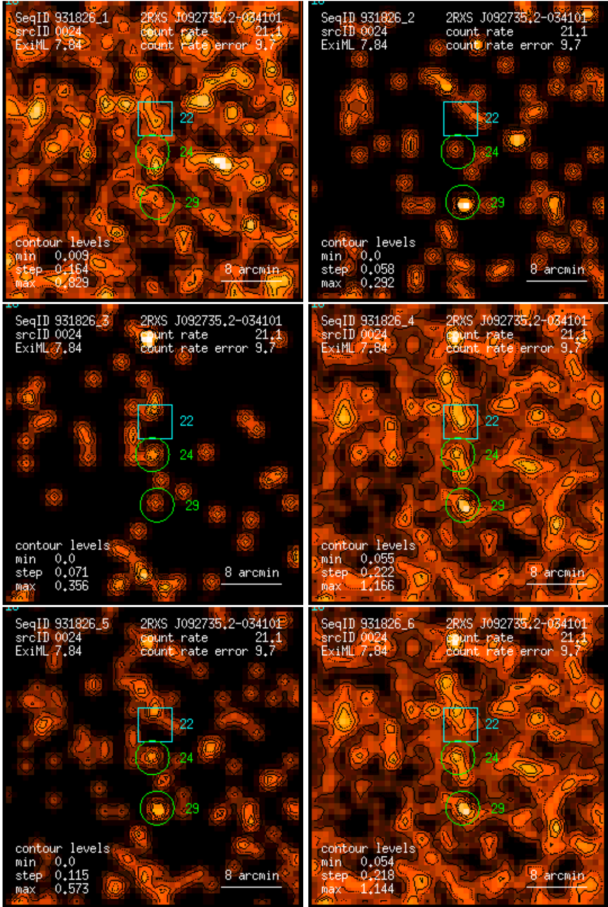
Figure 24: RASS 931826: detection 0024: band rate images, Gaussian filter: (1) PSPC channels 11 – 41, (2) 52 – 90, (3) 91 – 201, (4) 11 – 235, (5) 52 – 201, (6) 11 – 201. Broad band rates in counts/ks. Band rate contour levels in counts/ks/arcmin 2 .
