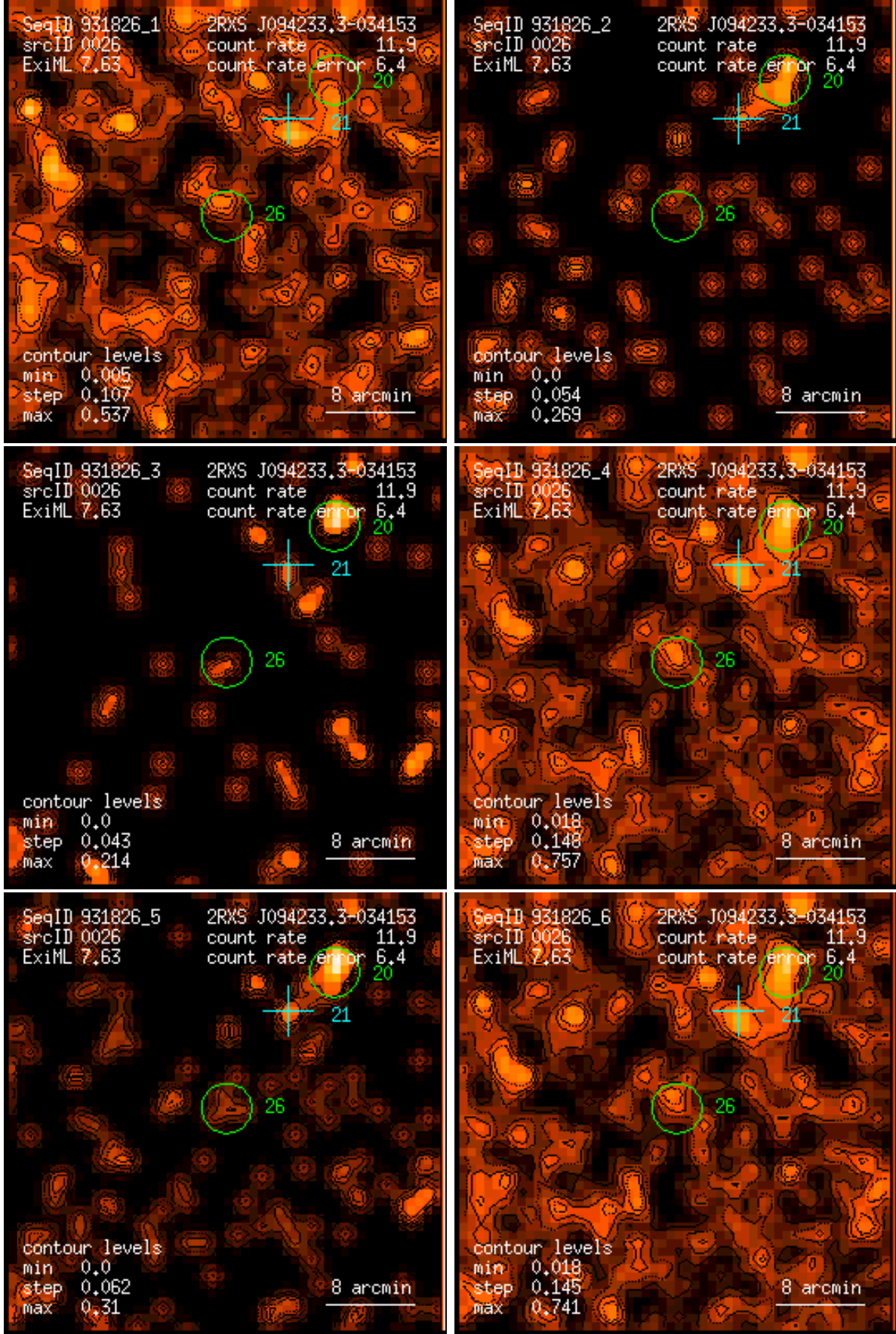
Figure 26: RASS 931826: detection 0026: band rate images, Gaussian filter: (1) PSPC channels 11 – 41, (2) 52 – 90, (3) 91 – 201, (4) 11 – 235, (5) 52 – 201, (6) 11 – 201. Broad band rates in counts/ks. Band rate contour levels in counts/ks/arcmin 2 .
