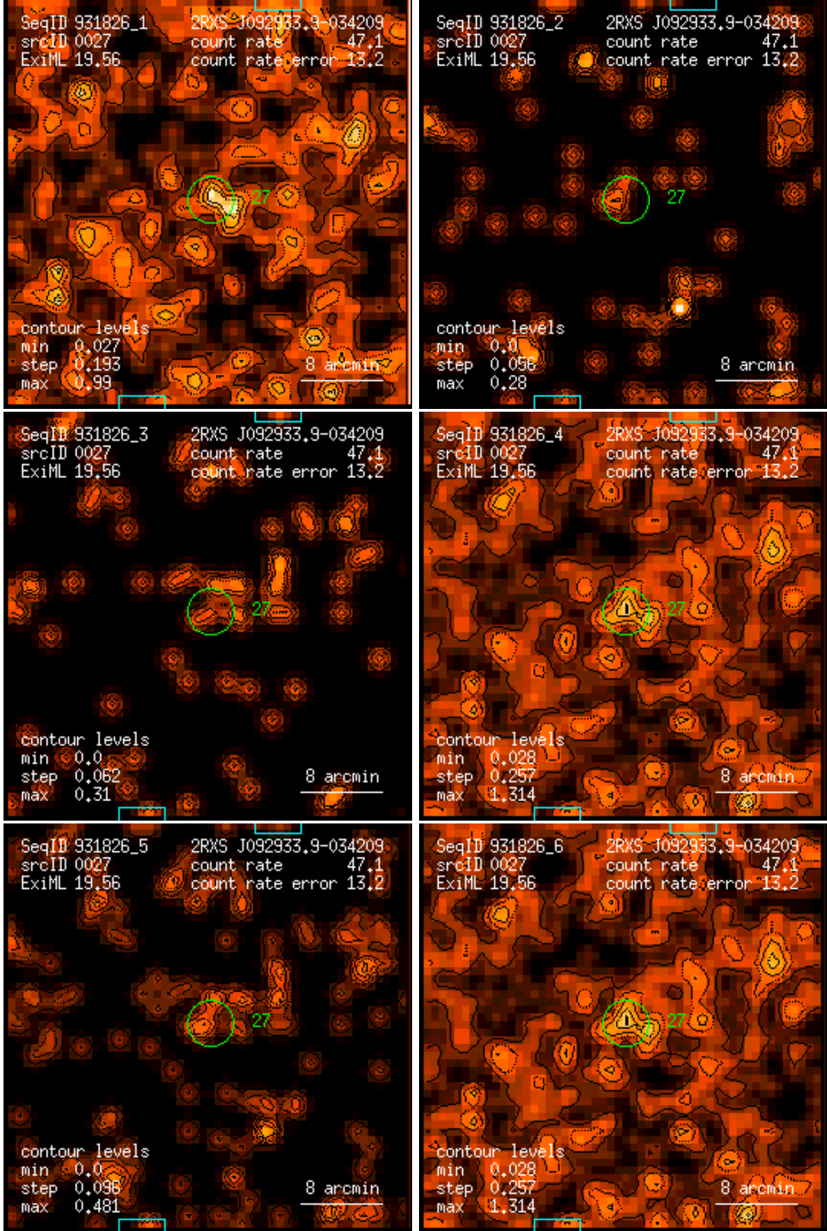
Figure 27: RASS 931826: detection 0027: band rate images, Gaussian filter: (1) PSPC channels 11 – 41, (2) 52 – 90, (3) 91 – 201, (4) 11 – 235, (5) 52 – 201, (6) 11 – 201. Broad band rates in counts/ks. Band rate contour levels in counts/ks/arcmin 2 .
