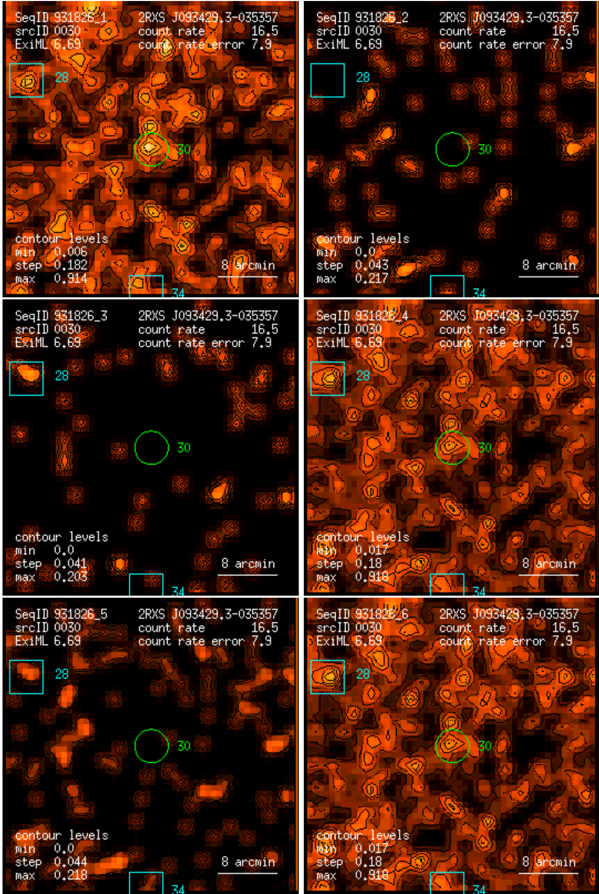
Figure 30: RASS 931826: detection 0030: band rate images, Gaussian filter: (1) PSPC channels 11 – 41, (2) 52 – 90, (3) 91 – 201, (4) 11 – 235, (5) 52 – 201, (6) 11 – 201. Broad band rates in counts/ks. Band rate contour levels in counts/ks/arcmin 2 .
