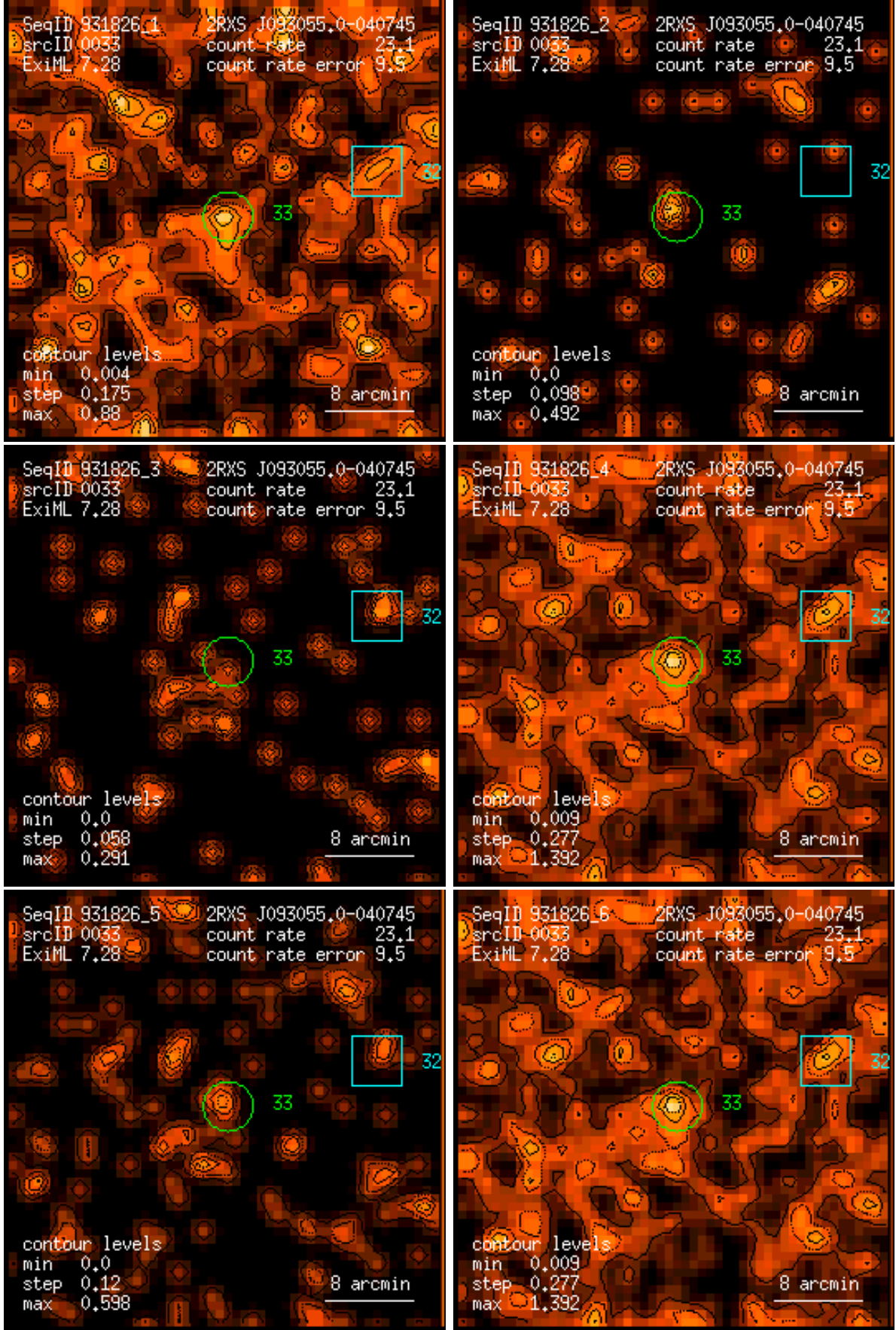
Figure 33: RASS 931826: detection 0033: band rate images, Gaussian filter: (1) PSPC channels 11 – 41, (2) 52 – 90, (3) 91 – 201, (4) 11 – 235, (5) 52 – 201, (6) 11 – 201. Broad band rates in counts/ks. Band rate contour levels in counts/ks/arcmin 2 .
