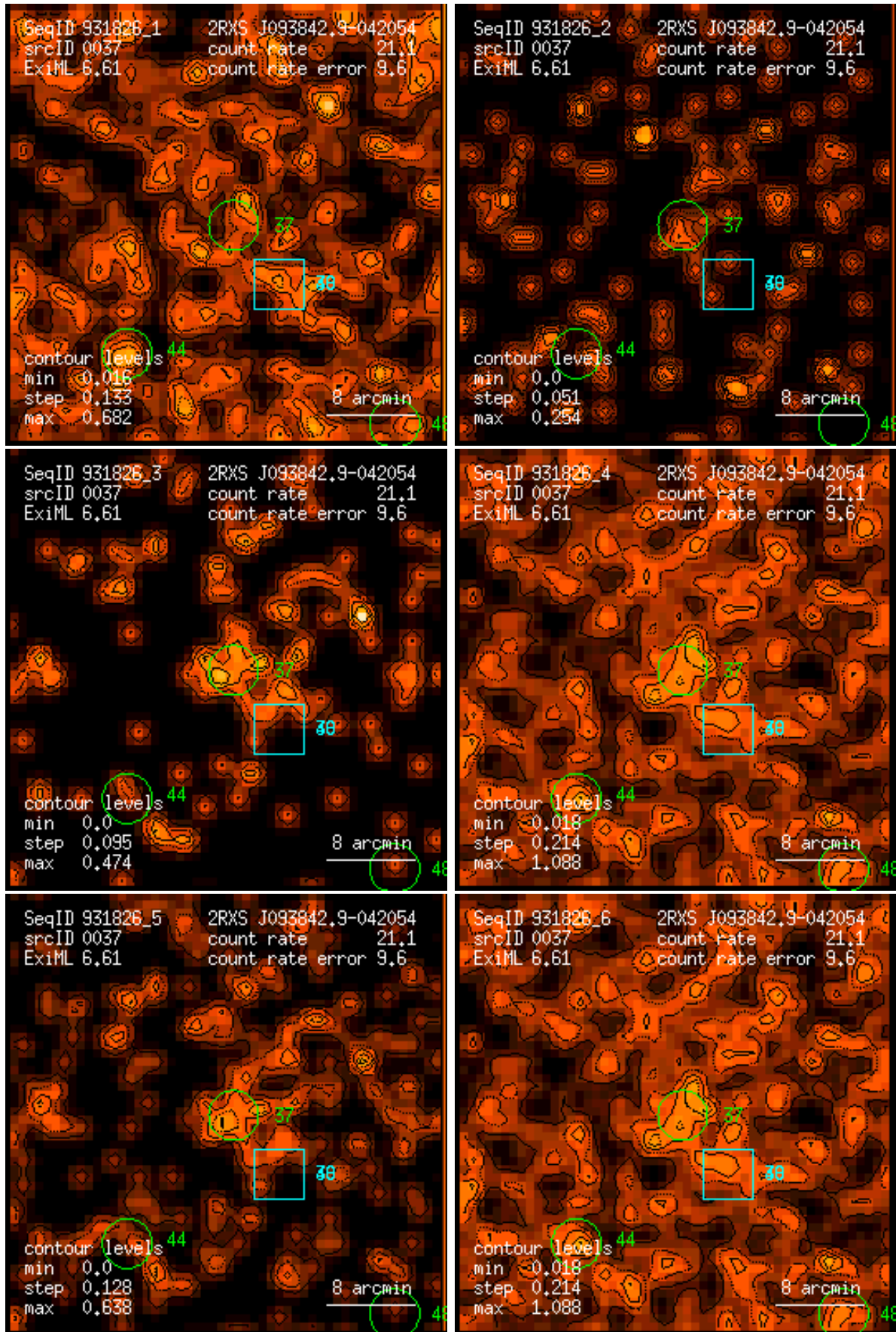
Figure 37: RASS 931826: detection 0037: band rate images, Gaussian filter: (1) PSPC channels 11 – 41, (2) 52 – 90, (3) 91 – 201, (4) 11 – 235, (5) 52 – 201, (6) 11 – 201. Broad band rates in counts/ks. Band rate contour levels in counts/ks/arcmin 2 .
