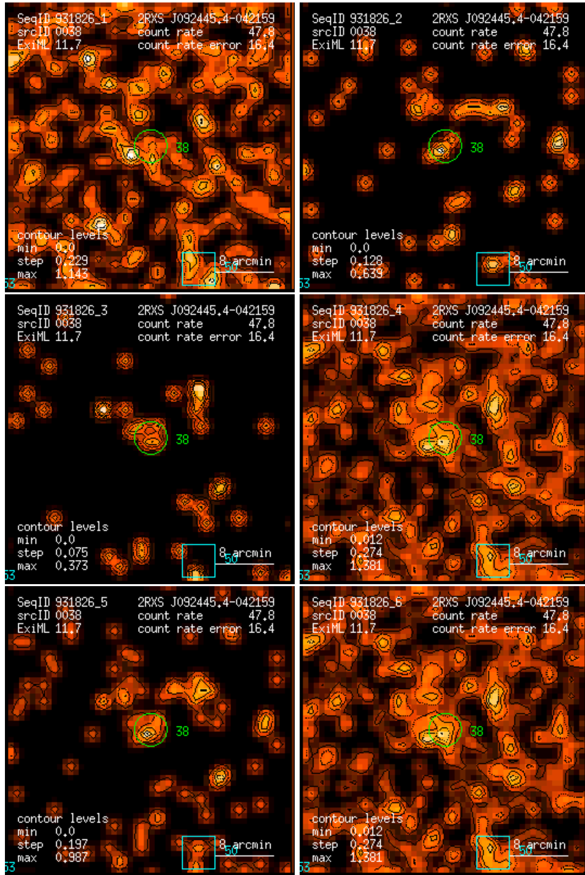
Figure 38: RASS 931826: detection 0038: band rate images, Gaussian filter: (1) PSPC channels 11 – 41, (2) 52 – 90, (3) 91 – 201, (4) 11 – 235, (5) 52 – 201, (6) 11 – 201. Broad band rates in counts/ks. Band rate contour levels in counts/ks/arcmin 2 .
