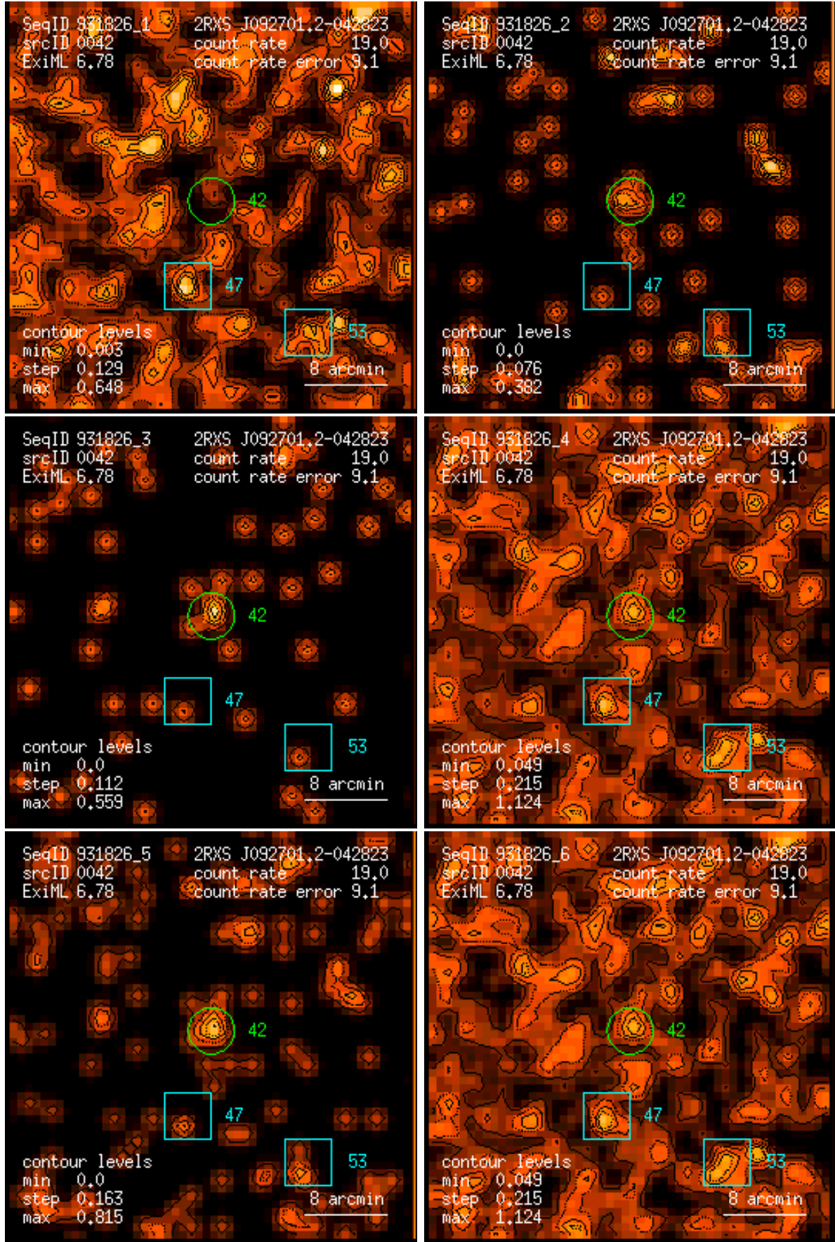
Figure 42: RASS 931826: detection 0042: band rate images, Gaussian filter: (1) PSPC channels 11 – 41, (2) 52 – 90, (3) 91 – 201, (4) 11 – 235, (5) 52 – 201, (6) 11 – 201. Broad band rates in counts/ks. Band rate contour levels in counts/ks/arcmin 2 .
