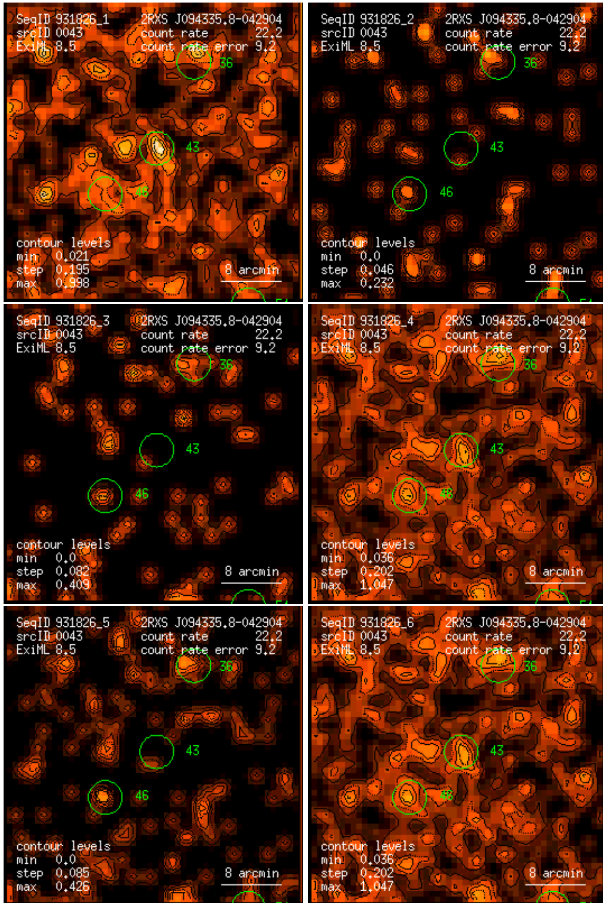
Figure 43: RASS 931826: detection 0043: band rate images, Gaussian filter: (1) PSPC channels 11 – 41, (2) 52 – 90, (3) 91 – 201, (4) 11 – 235, (5) 52 – 201, (6) 11 – 201. Broad band rates in counts/ks. Band rate contour levels in counts/ks/arcmin 2 .
