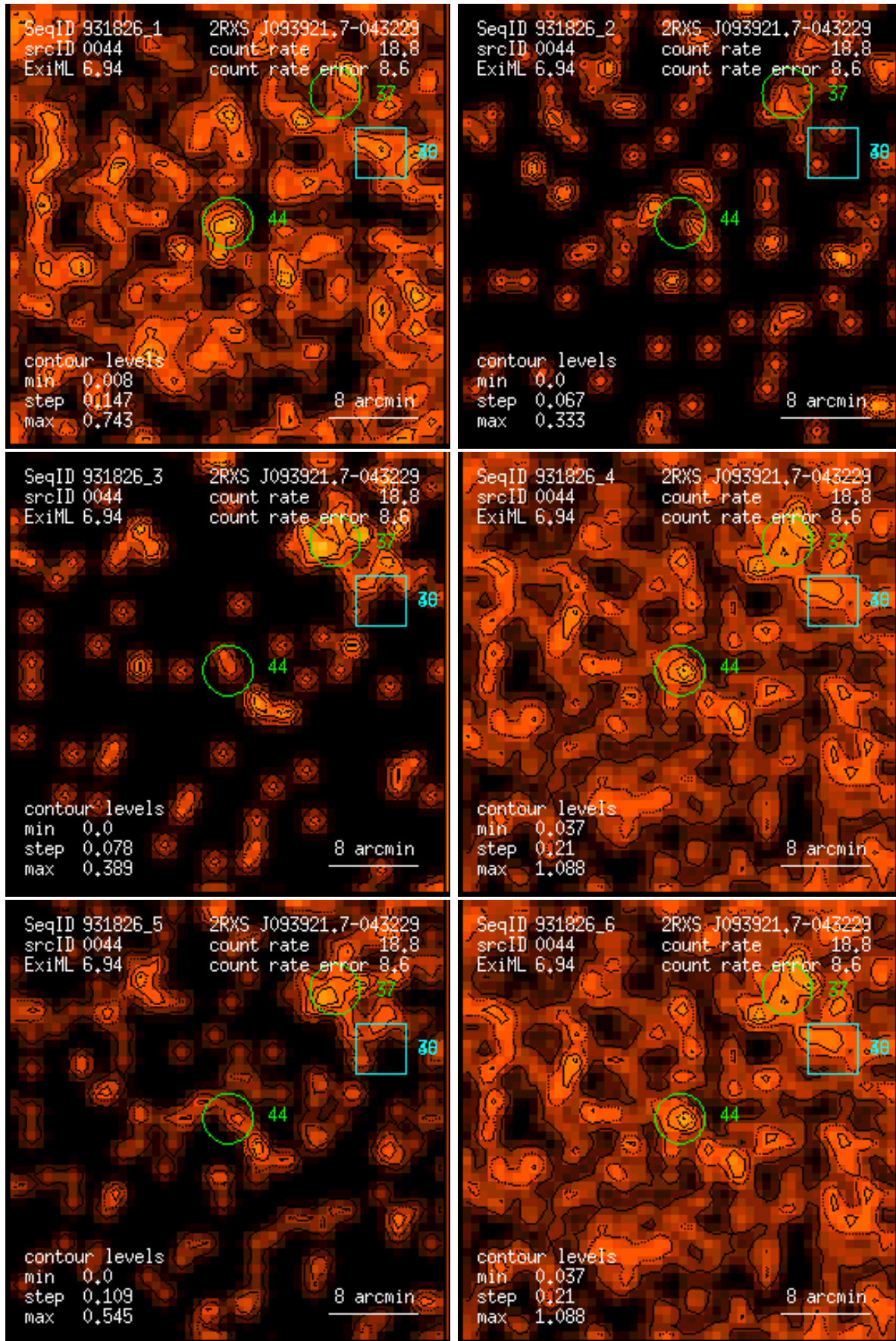
Figure 44: RASS 931826: detection 0044: band rate images, Gaussian filter: (1) PSPC channels 11 – 41, (2) 52 – 90, (3) 91 – 201, (4) 11 – 235, (5) 52 – 201, (6) 11 – 201. Broad band rates in counts/ks. Band rate contour levels in counts/ks/arcmin 2 .
