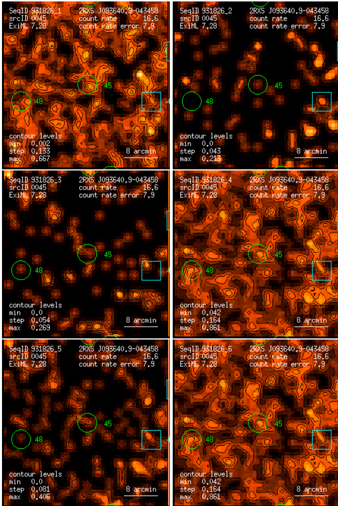
Figure 45: RASS 931826: detection 0045: band rate images, Gaussian filter: (1) PSPC channels 11 – 41, (2) 52 – 90, (3) 91 – 201, (4) 11 – 235, (5) 52 – 201, (6) 11 – 201. Broad band rates in counts/ks. Band rate contour levels in counts/ks/arcmin 2 .
