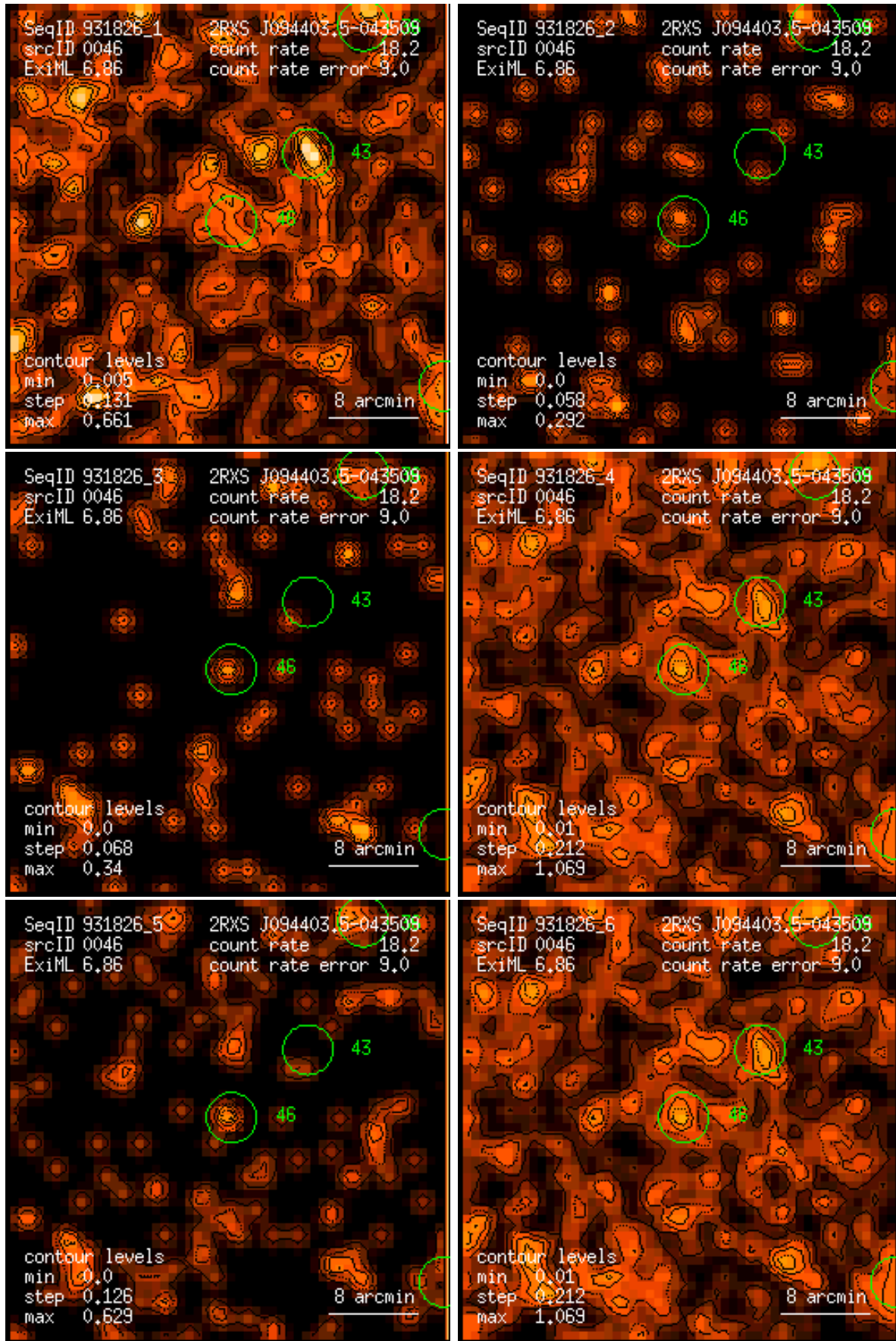
Figure 46: RASS 931826: detection 0046: band rate images, Gaussian filter: (1) PSPC channels 11 – 41, (2) 52 – 90, (3) 91 – 201, (4) 11 – 235, (5) 52 – 201, (6) 11 – 201. Broad band rates in counts/ks. Band rate contour levels in counts/ks/arcmin 2 .
