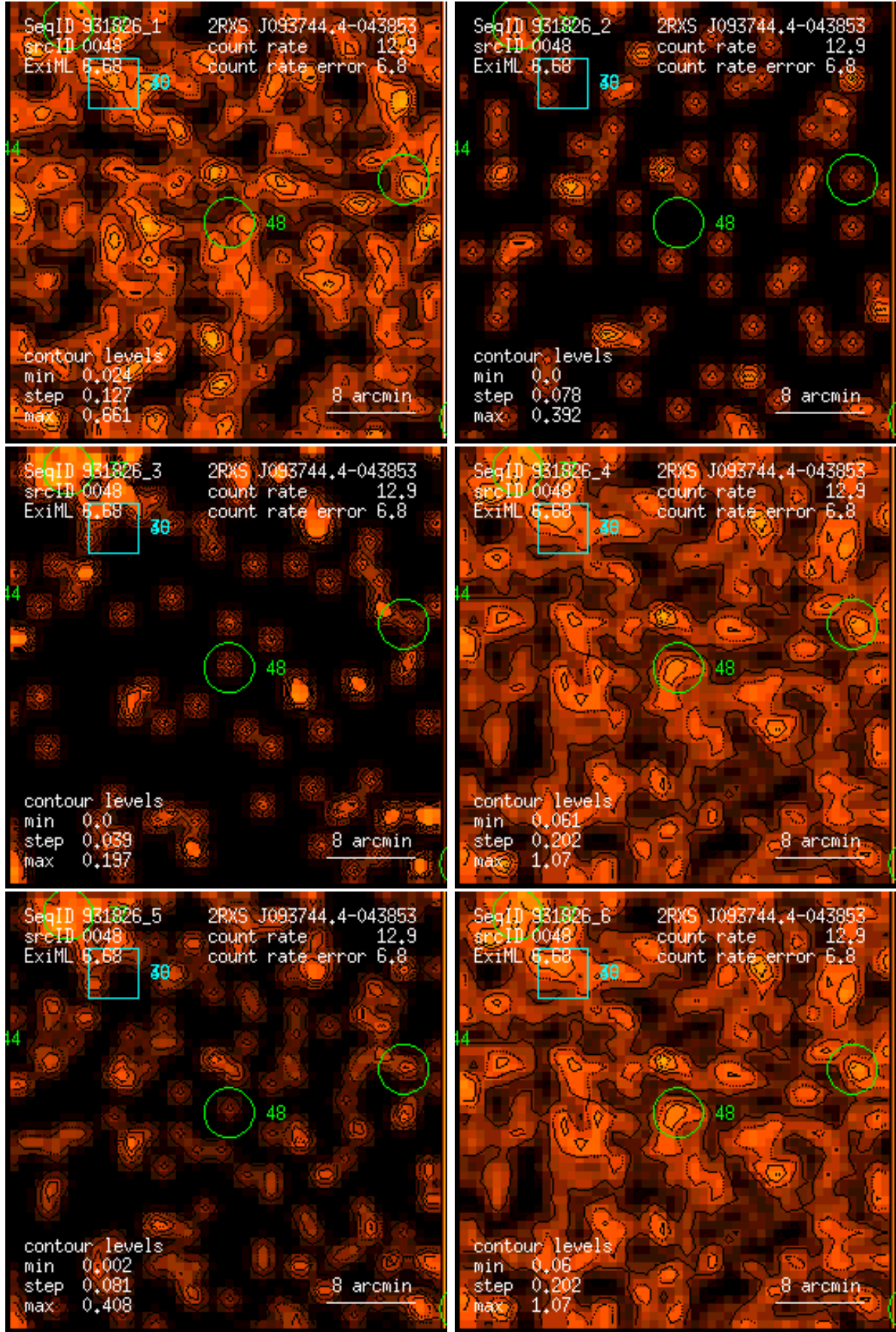
Figure 48: RASS 931826: detection 0048: band rate images, Gaussian filter: (1) PSPC channels 11 – 41, (2) 52 – 90, (3) 91 – 201, (4) 11 – 235, (5) 52 – 201, (6) 11 – 201. Broad band rates in counts/ks. Band rate contour levels in counts/ks/arcmin 2 .
