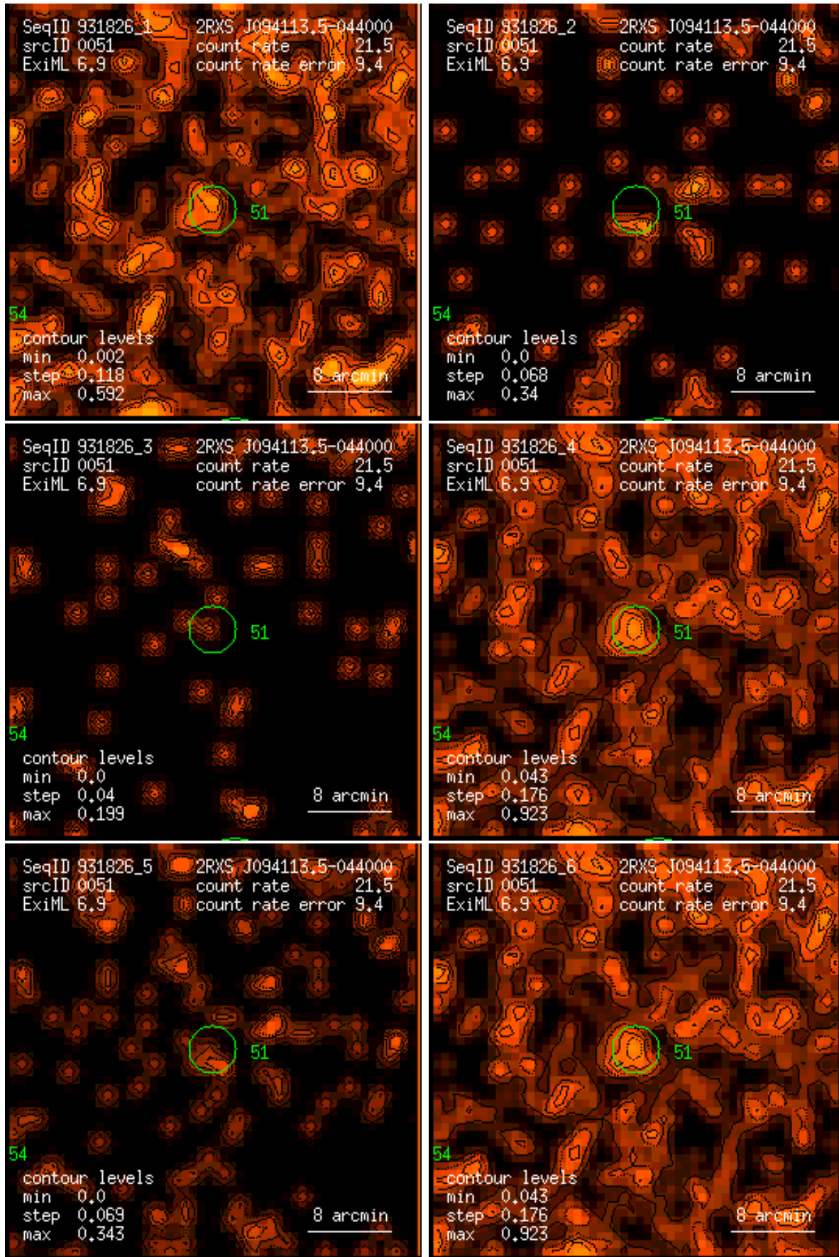
Figure 51: RASS 931826: detection 0051: band rate images, Gaussian filter: (1) PSPC channels 11 – 41, (2) 52 – 90, (3) 91 – 201, (4) 11 – 235, (5) 52 – 201, (6) 11 – 201. Broad band rates in counts/ks. Band rate contour levels in counts/ks/arcmin 2 .
