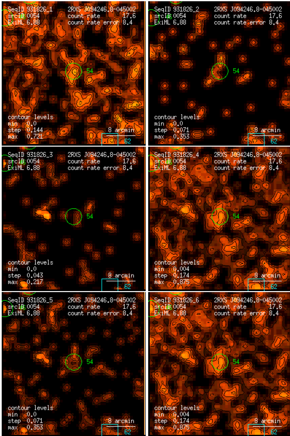
Figure 54: RASS 931826: detection 0054: band rate images, Gaussian filter: (1) PSPC channels 11 – 41, (2) 52 – 90, (3) 91 – 201, (4) 11 – 235, (5) 52 – 201, (6) 11 – 201. Broad band rates in counts/ks. Band rate contour levels in counts/ks/arcmin 2 .
