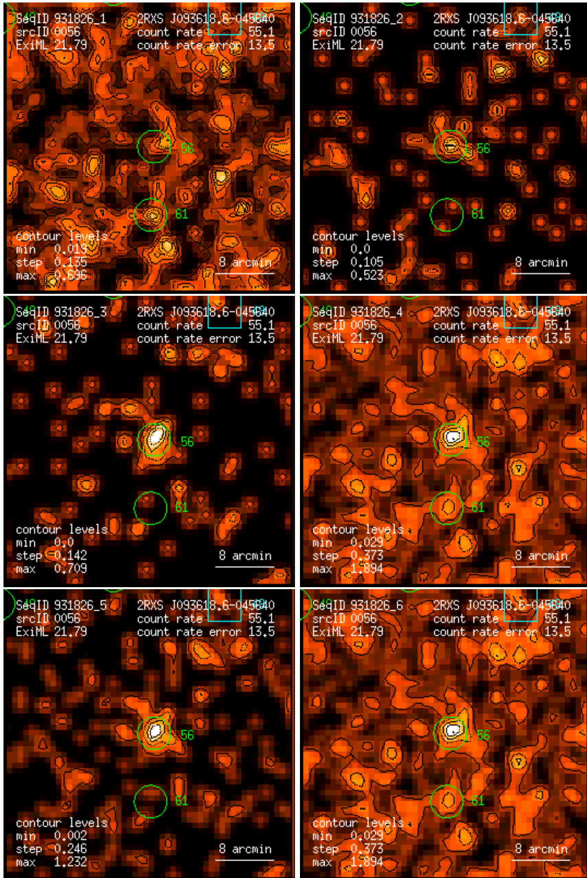
Figure 56: RASS 931826: detection 0056: band rate images, Gaussian filter: (1) PSPC channels 11 – 41, (2) 52 – 90, (3) 91 – 201, (4) 11 – 235, (5) 52 – 201, (6) 11 – 201. Broad band rates in counts/ks. Band rate contour levels in counts/ks/arcmin 2 .
