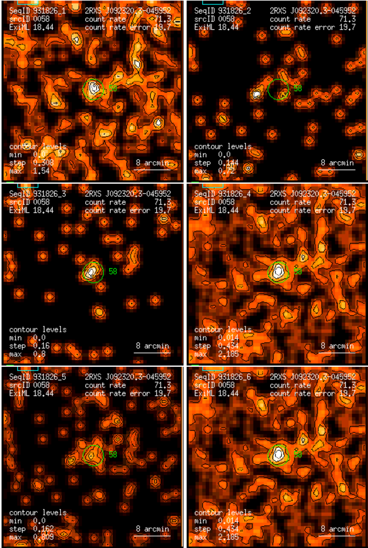
Figure 58: RASS 931826: detection 0058: band rate images, Gaussian filter: (1) PSPC channels 11 – 41, (2) 52 – 90, (3) 91 – 201, (4) 11 – 235, (5) 52 – 201, (6) 11 – 201. Broad band rates in counts/ks. Band rate contour levels in counts/ks/arcmin 2 .
