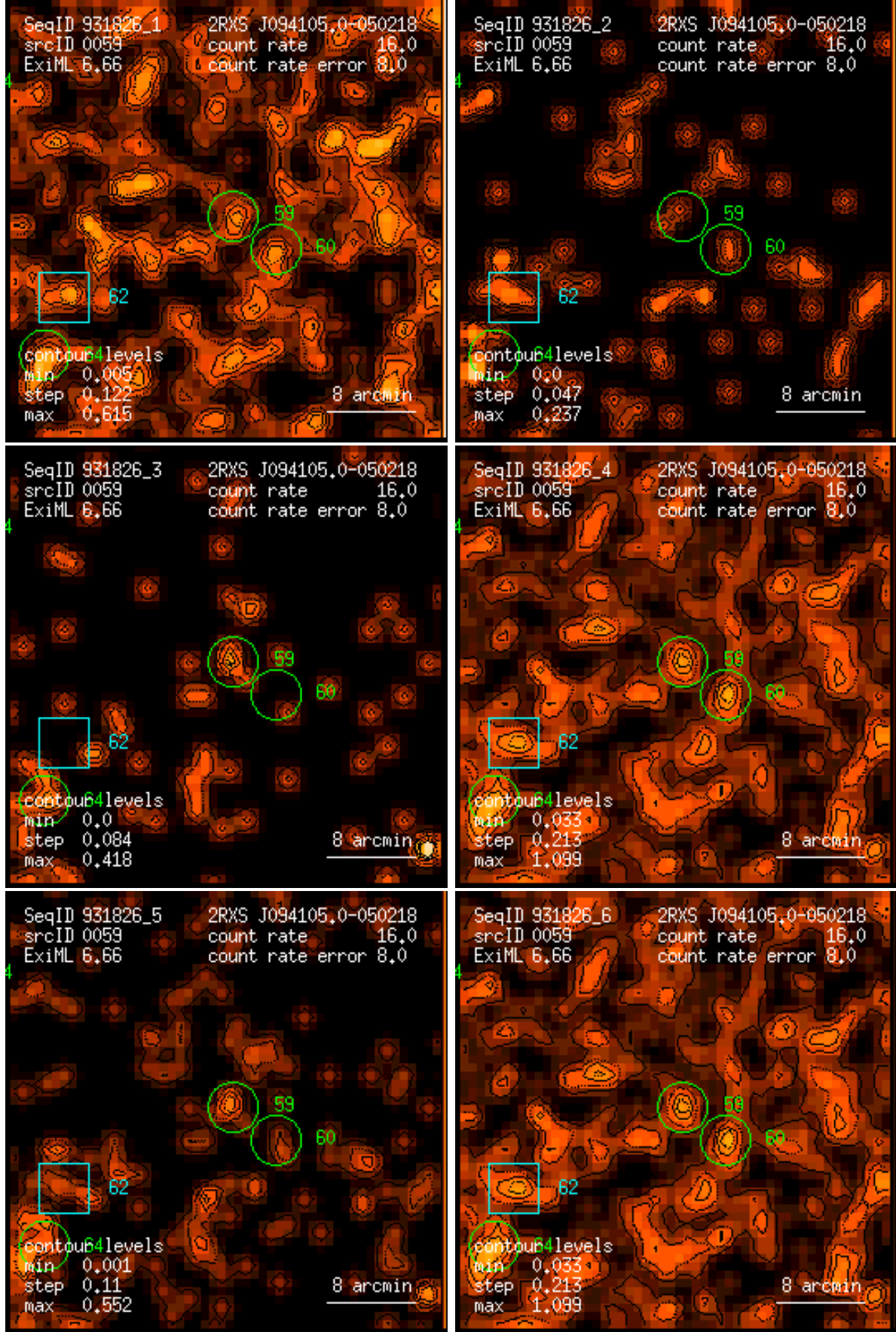
Figure 59: RASS 931826: detection 0059: band rate images, Gaussian filter: (1) PSPC channels 11 – 41, (2) 52 – 90, (3) 91 – 201, (4) 11 – 235, (5) 52 – 201, (6) 11 – 201. Broad band rates in counts/ks. Band rate contour levels in counts/ks/arcmin 2 .
