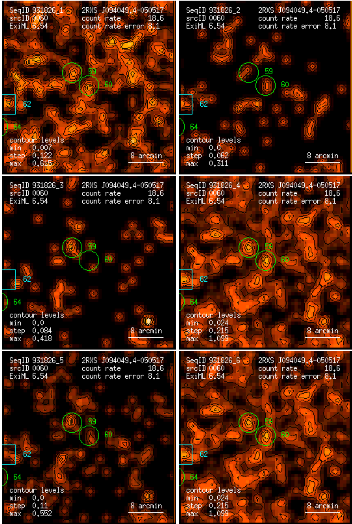
Figure 60: RASS 931826: detection 0060: band rate images, Gaussian filter: (1) PSPC channels 11 – 41, (2) 52 – 90, (3) 91 – 201, (4) 11 – 235, (5) 52 – 201, (6) 11 – 201. Broad band rates in counts/ks. Band rate contour levels in counts/ks/arcmin 2 .
