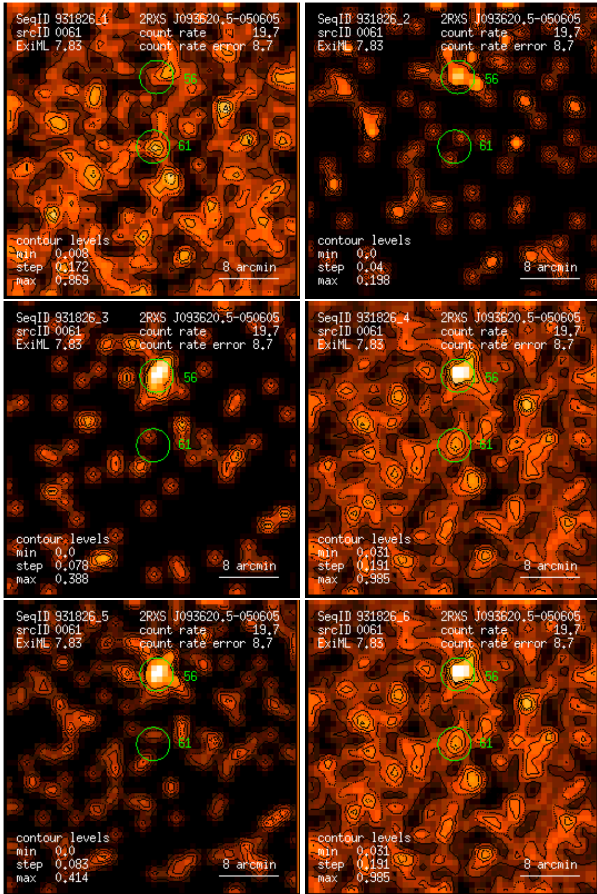
Figure 61: RASS 931826: detection 0061: band rate images, Gaussian filter: (1) PSPC channels 11 – 41, (2) 52 – 90, (3) 91 – 201, (4) 11 – 235, (5) 52 – 201, (6) 11 – 201. Broad band rates in counts/ks. Band rate contour levels in counts/ks/arcmin 2 .
