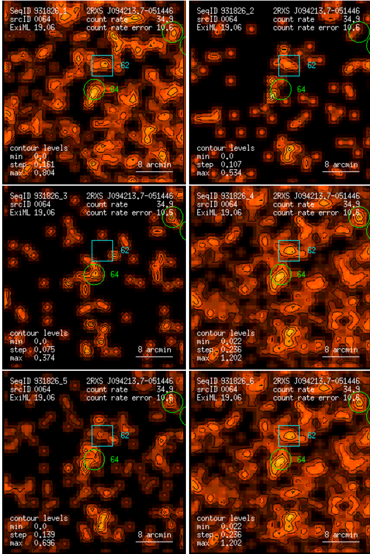
Figure 64: RASS 931826: detection 0064: band rate images, Gaussian filter: (1) PSPC channels 11 – 41, (2) 52 – 90, (3) 91 – 201, (4) 11 – 235, (5) 52 – 201, (6) 11 – 201. Broad band rates in counts/ks. Band rate contour levels in counts/ks/arcmin 2 .
