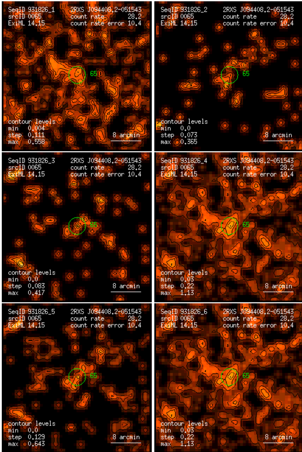
Figure 65: RASS 931826: detection 0065: band rate images, Gaussian filter: (1) PSPC channels 11 – 41, (2) 52 – 90, (3) 91 – 201, (4) 11 – 235, (5) 52 – 201, (6) 11 – 201. Broad band rates in counts/ks. Band rate contour levels in counts/ks/arcmin 2 .
