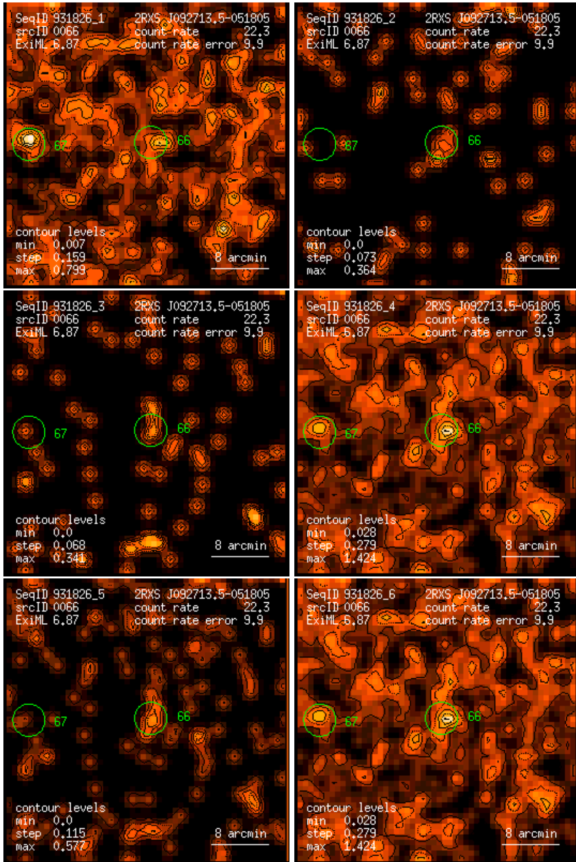
Figure 66: RASS 931826: detection 0066: band rate images, Gaussian filter: (1) PSPC channels 11 – 41, (2) 52 – 90, (3) 91 – 201, (4) 11 – 235, (5) 52 – 201, (6) 11 – 201. Broad band rates in counts/ks. Band rate contour levels in counts/ks/arcmin 2 .
