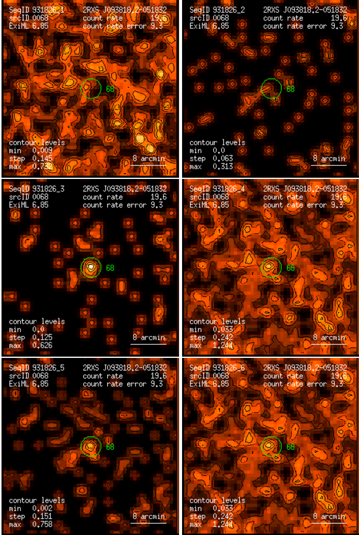
Figure 68: RASS 931826: detection 0068: band rate images, Gaussian filter: (1) PSPC channels 11 – 41, (2) 52 – 90, (3) 91 – 201, (4) 11 – 235, (5) 52 – 201, (6) 11 – 201. Broad band rates in counts/ks. Band rate contour levels in counts/ks/arcmin 2 .
