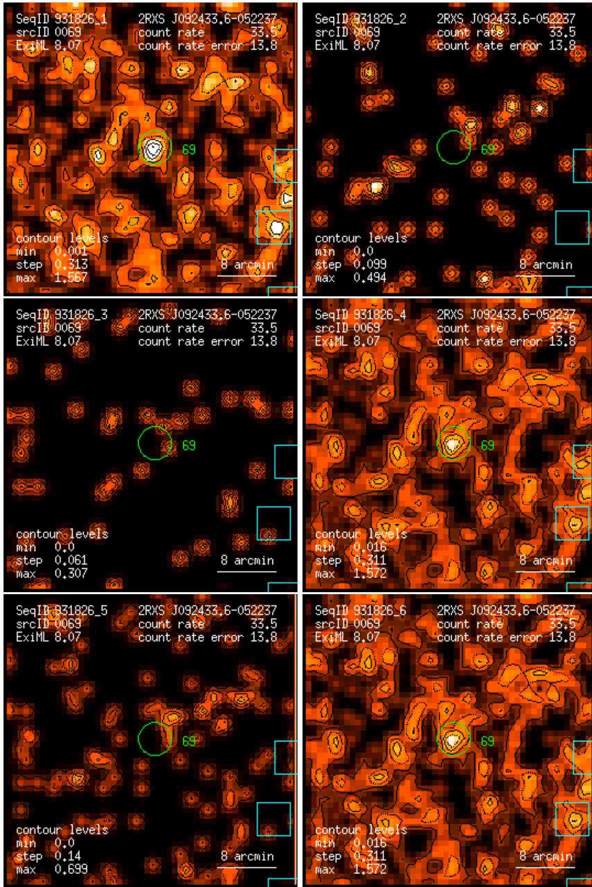
Figure 69: RASS 931826: detection 0069: band rate images, Gaussian filter: (1) PSPC channels 11 – 41, (2) 52 – 90, (3) 91 – 201, (4) 11 – 235, (5) 52 – 201, (6) 11 – 201. Broad band rates in counts/ks. Band rate contour levels in counts/ks/arcmin 2 .
