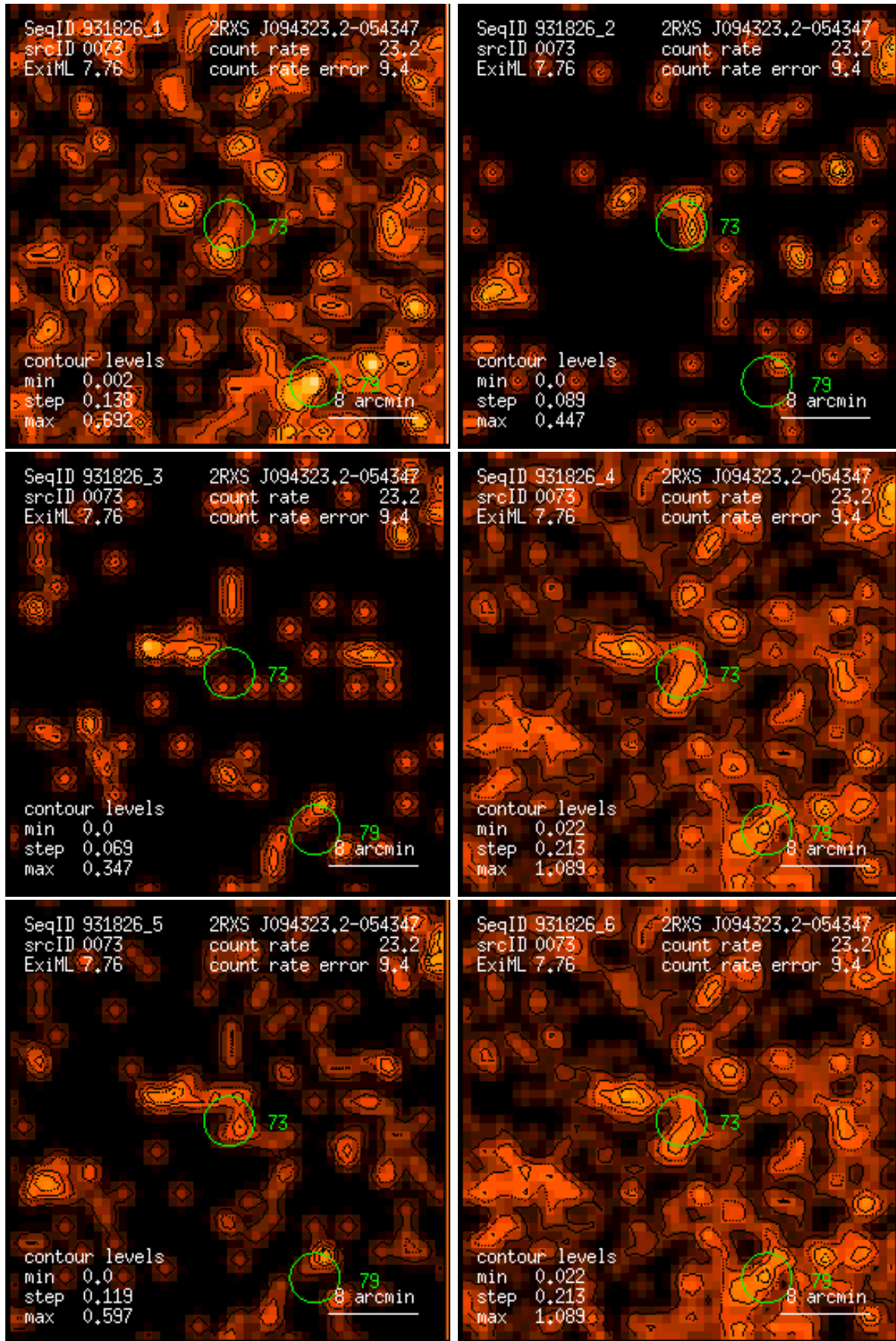
Figure 73: RASS 931826: detection 0073: band rate images, Gaussian filter: (1) PSPC channels 11 – 41, (2) 52 – 90, (3) 91 – 201, (4) 11 – 235, (5) 52 – 201, (6) 11 – 201. Broad band rates in counts/ks. Band rate contour levels in counts/ks/arcmin 2 .
