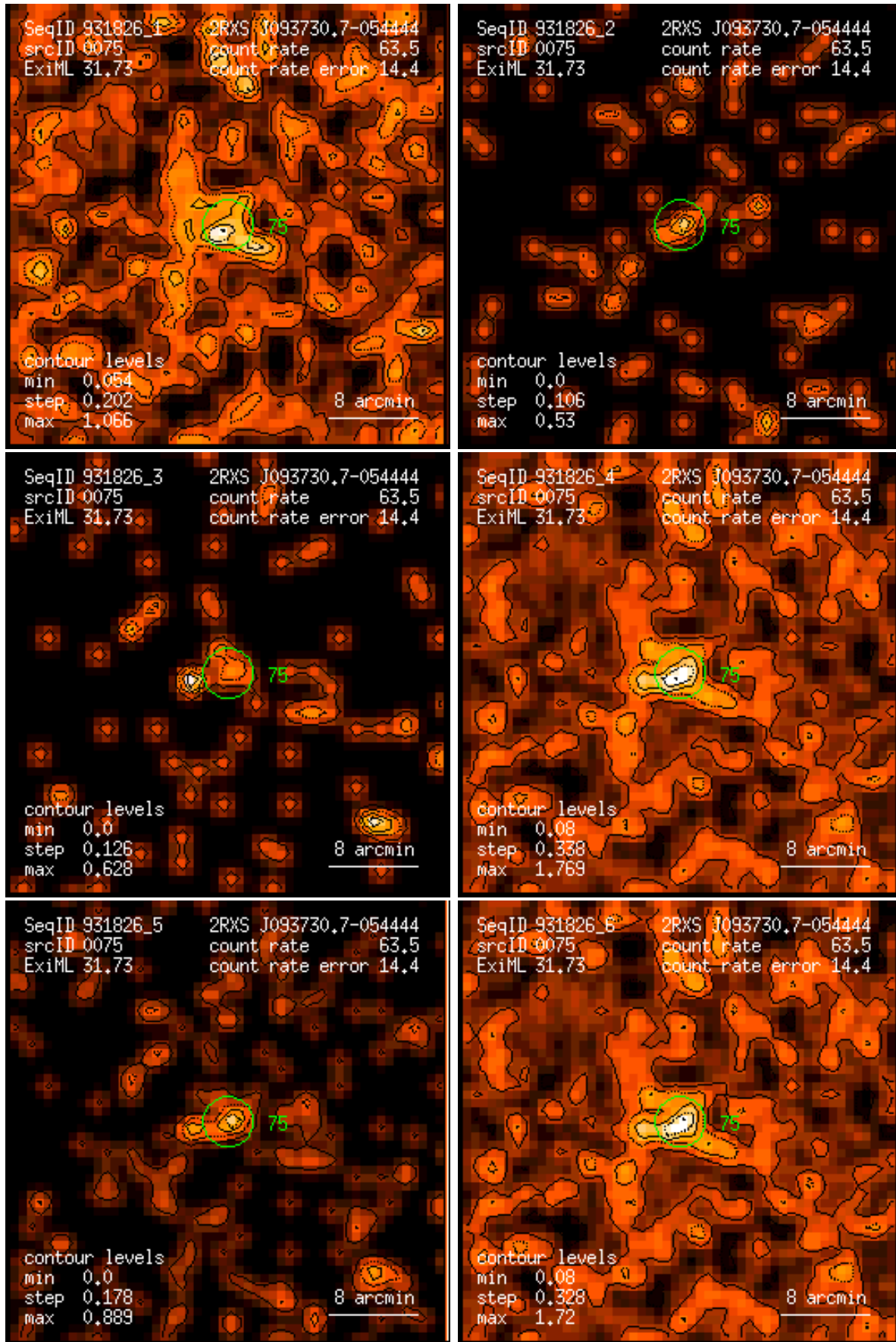
Figure 75: RASS 931826: detection 0075: band rate images, Gaussian filter: (1) PSPC channels 11 – 41, (2) 52 – 90, (3) 91 – 201, (4) 11 – 235, (5) 52 – 201, (6) 11 – 201. Broad band rates in counts/ks. Band rate contour levels in counts/ks/arcmin 2 .
