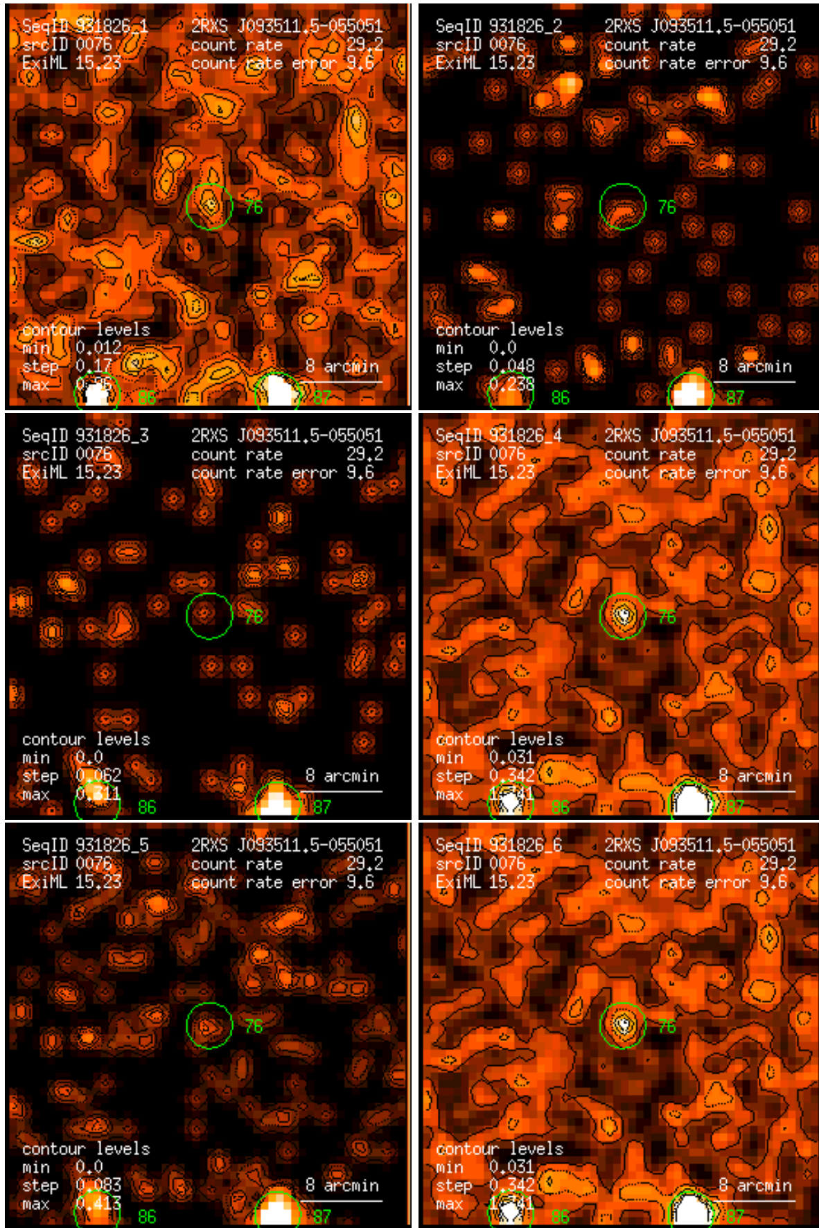
Figure 76: RASS 931826: detection 0076: band rate images, Gaussian filter: (1) PSPC channels 11 – 41, (2) 52 – 90, (3) 91 – 201, (4) 11 – 235, (5) 52 – 201, (6) 11 – 201. Broad band rates in counts/ks. Band rate contour levels in counts/ks/arcmin 2 .
