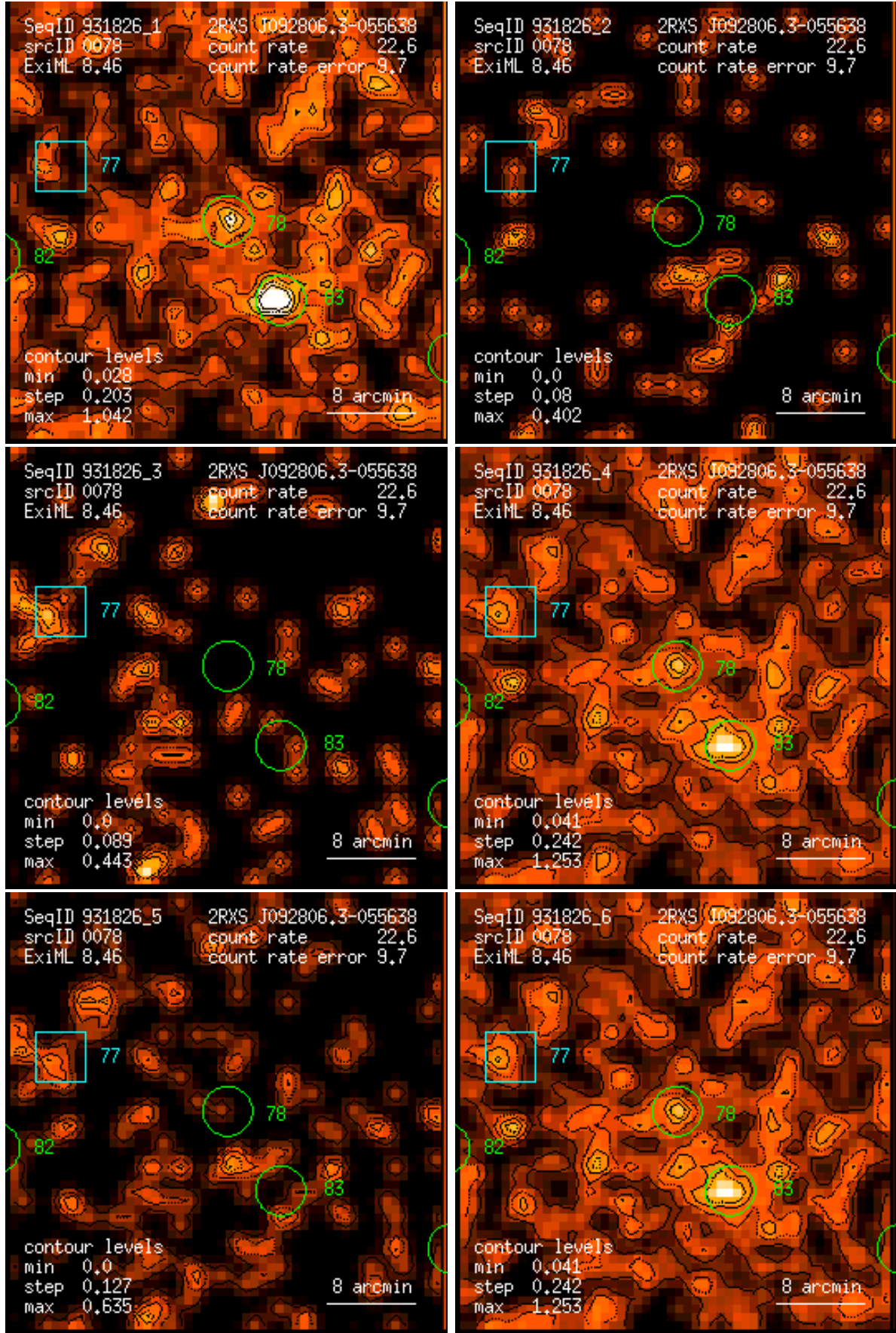
Figure 78: RASS 931826: detection 0078: band rate images, Gaussian filter: (1) PSPC channels 11 – 41, (2) 52 – 90, (3) 91 – 201, (4) 11 – 235, (5) 52 – 201, (6) 11 – 201. Broad band rates in counts/ks. Band rate contour levels in counts/ks/arcmin 2 .
