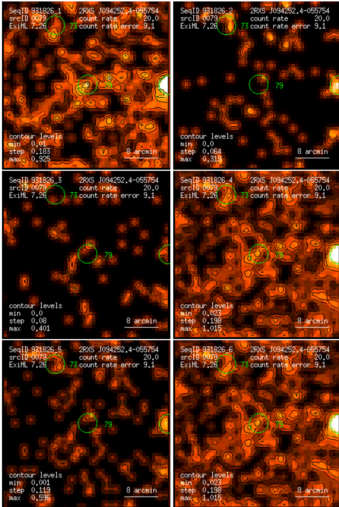
Figure 79: RASS 931826: detection 0079: band rate images, Gaussian filter: (1) PSPC channels 11 – 41, (2) 52 – 90, (3) 91 – 201, (4) 11 – 235, (5) 52 – 201, (6) 11 – 201. Broad band rates in counts/ks. Band rate contour levels in counts/ks/arcmin 2 .
