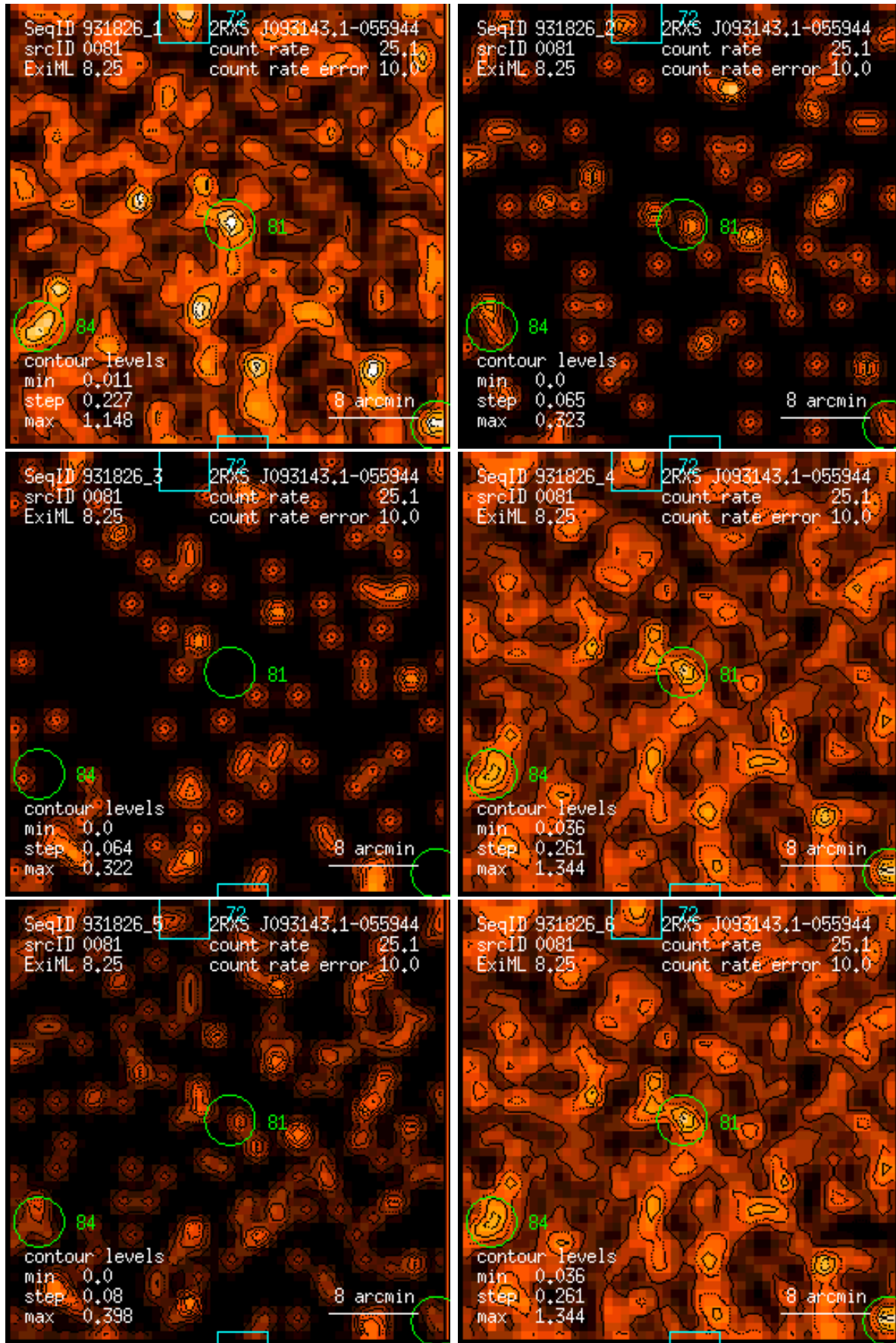
Figure 81: RASS 931826: detection 0081: band rate images, Gaussian filter: (1) PSPC channels 11 – 41, (2) 52 – 90, (3) 91 – 201, (4) 11 – 235, (5) 52 – 201, (6) 11 – 201. Broad band rates in counts/ks. Band rate contour levels in counts/ks/arcmin 2 .
