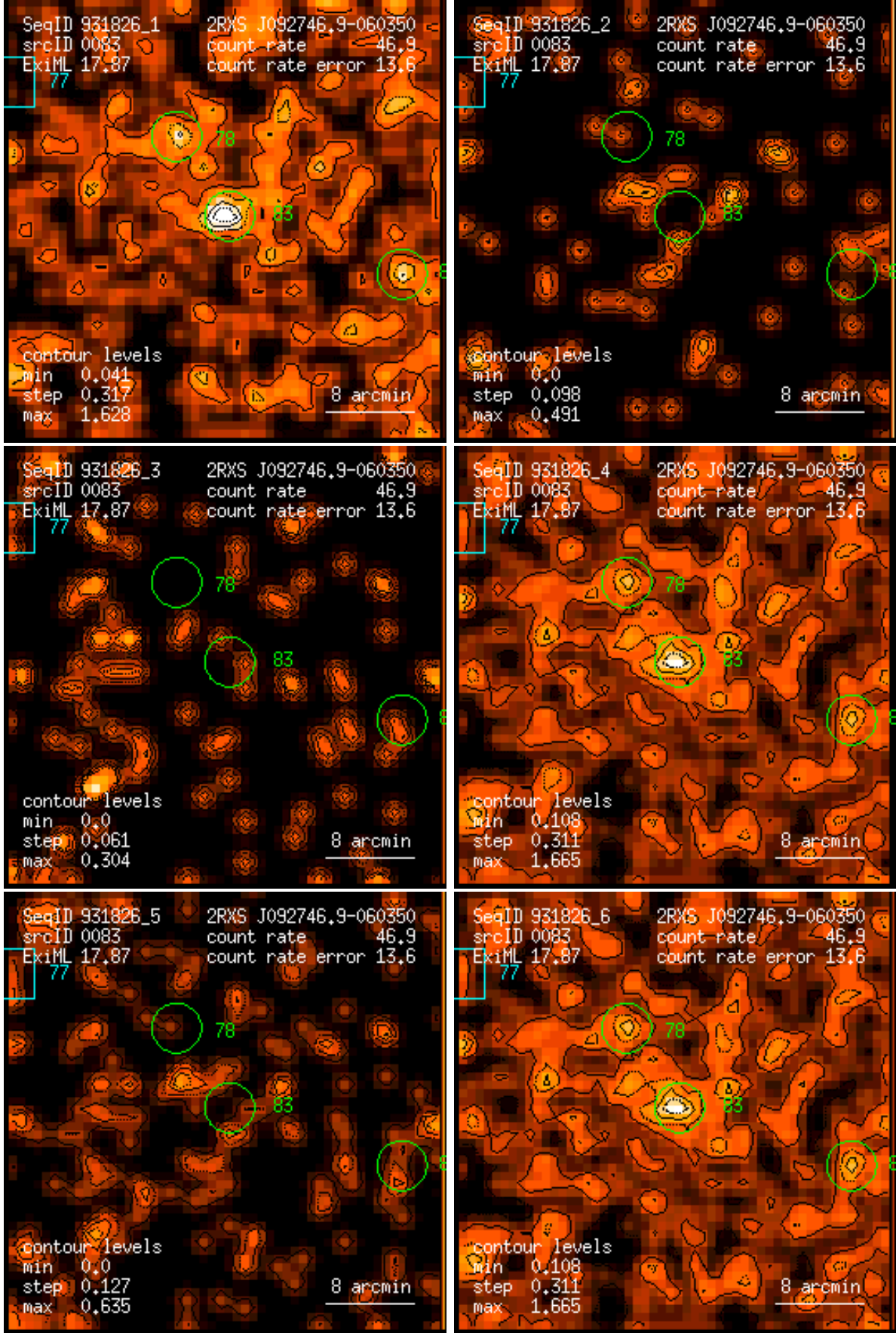
Figure 83: RASS 931826: detection 0083: band rate images, Gaussian filter: (1) PSPC channels 11 – 41, (2) 52 – 90, (3) 91 – 201, (4) 11 – 235, (5) 52 – 201, (6) 11 – 201. Broad band rates in counts/ks. Band rate contour levels in counts/ks/arcmin 2 .
