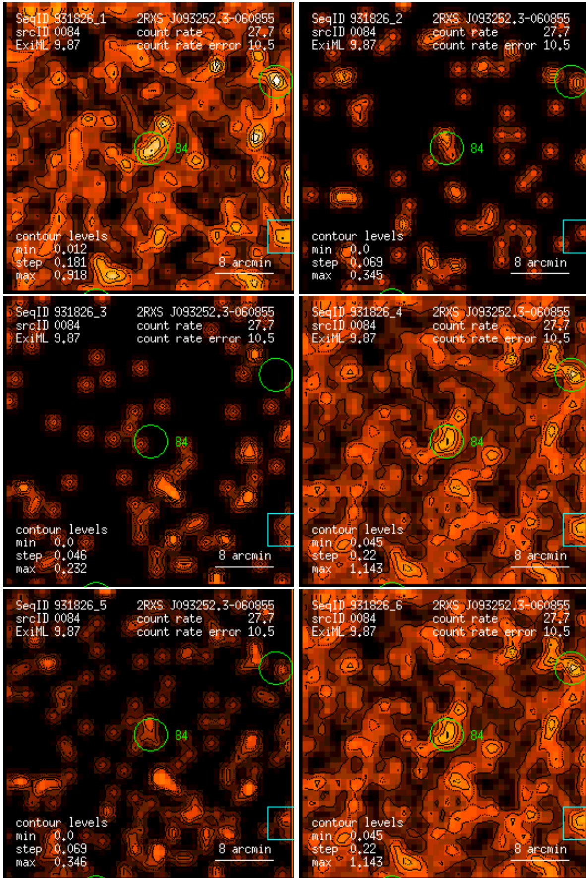
Figure 84: RASS 931826: detection 0084: band rate images, Gaussian filter: (1) PSPC channels 11 – 41, (2) 52 – 90, (3) 91 – 201, (4) 11 – 235, (5) 52 – 201, (6) 11 – 201. Broad band rates in counts/ks. Band rate contour levels in counts/ks/arcmin 2 .
