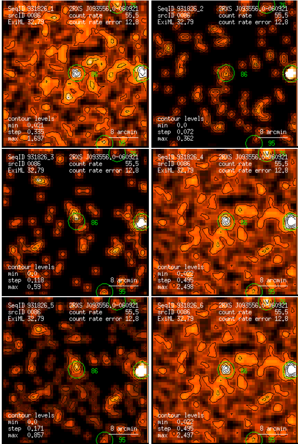
Figure 86: RASS 931826: detection 0086: band rate images, Gaussian filter: (1) PSPC channels 11 – 41, (2) 52 – 90, (3) 91 – 201, (4) 11 – 235, (5) 52 – 201, (6) 11 – 201. Broad band rates in counts/ks. Band rate contour levels in counts/ks/arcmin 2 .
