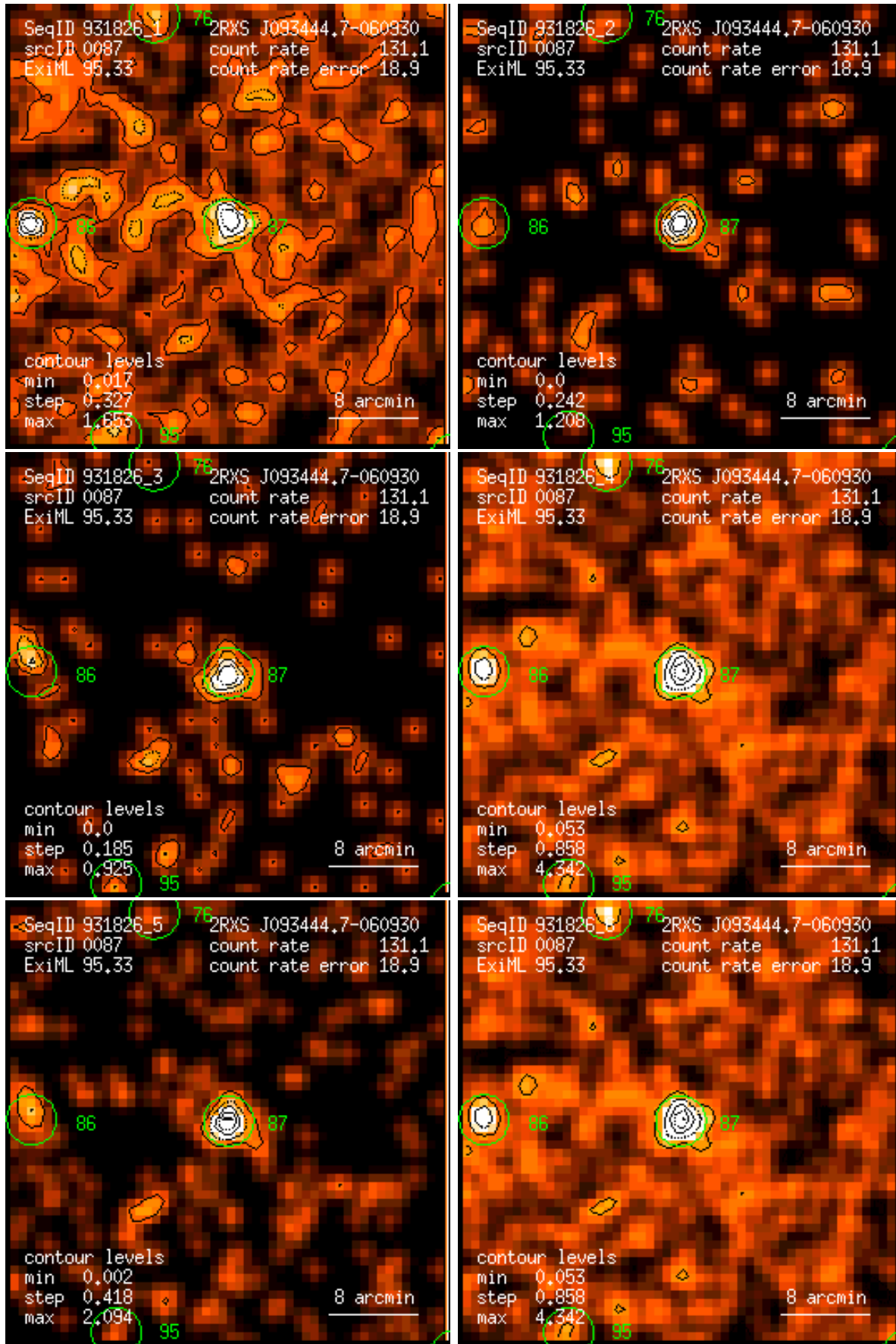
Figure 87: RASS 931826: detection 0087: band rate images, Gaussian filter: (1) PSPC channels 11 – 41, (2) 52 – 90, (3) 91 – 201, (4) 11 – 235, (5) 52 – 201, (6) 11 – 201. Broad band rates in counts/ks. Band rate contour levels in counts/ks/arcmin 2 .
