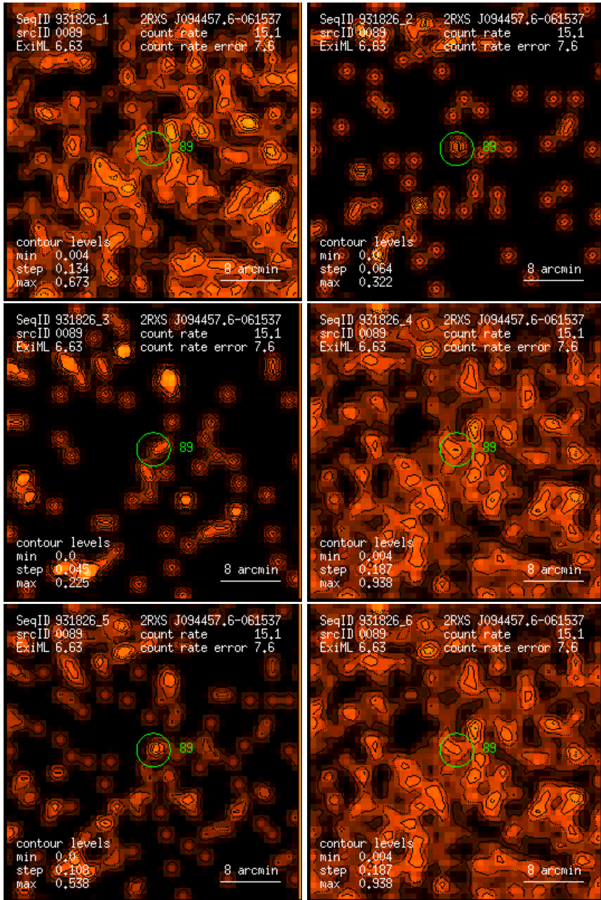
Figure 89: RASS 931826: detection 0089: band rate images, Gaussian filter: (1) PSPC channels 11 – 41, (2) 52 – 90, (3) 91 – 201, (4) 11 – 235, (5) 52 – 201, (6) 11 – 201. Broad band rates in counts/ks. Band rate contour levels in counts/ks/arcmin 2 .
