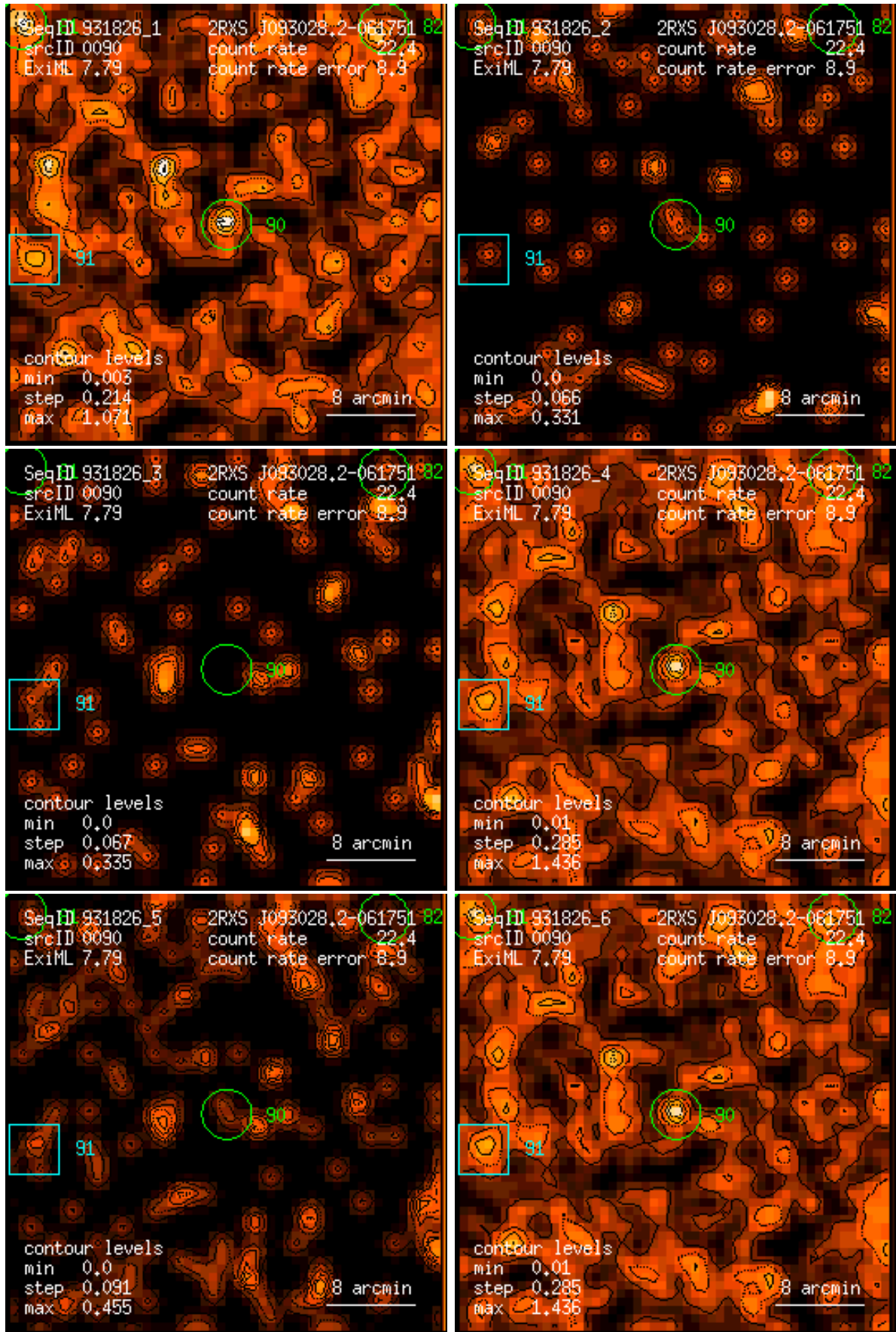
Figure 90: RASS 931826: detection 0090: band rate images, Gaussian filter: (1) PSPC channels 11 – 41, (2) 52 – 90, (3) 91 – 201, (4) 11 – 235, (5) 52 – 201, (6) 11 – 201. Broad band rates in counts/ks. Band rate contour levels in counts/ks/arcmin 2 .
