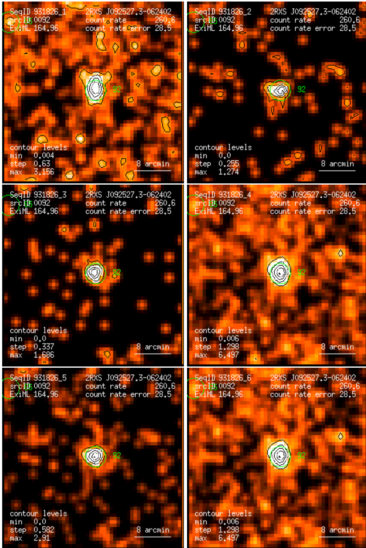
Figure 92: RASS 931826: detection 0092: band rate images, Gaussian filter: (1) PSPC channels 11 – 41, (2) 52 – 90, (3) 91 – 201, (4) 11 – 235, (5) 52 – 201, (6) 11 – 201. Broad band rates in counts/ks. Band rate contour levels in counts/ks/arcmin 2 .
