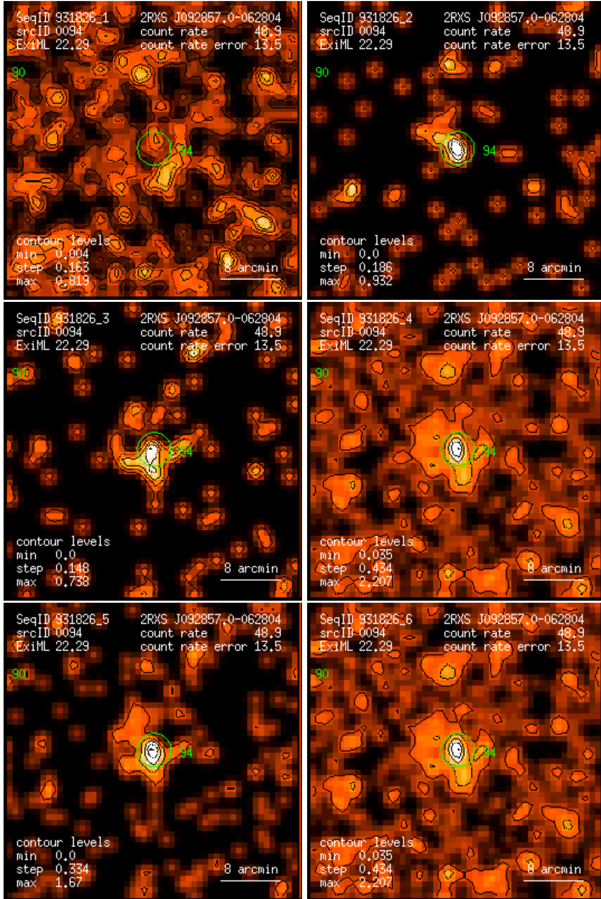
Figure 94: RASS 931826: detection 0094: band rate images, Gaussian filter: (1) PSPC channels 11 – 41, (2) 52 – 90, (3) 91 – 201, (4) 11 – 235, (5) 52 – 201, (6) 11 – 201. Broad band rates in counts/ks. Band rate contour levels in counts/ks/arcmin 2 .
