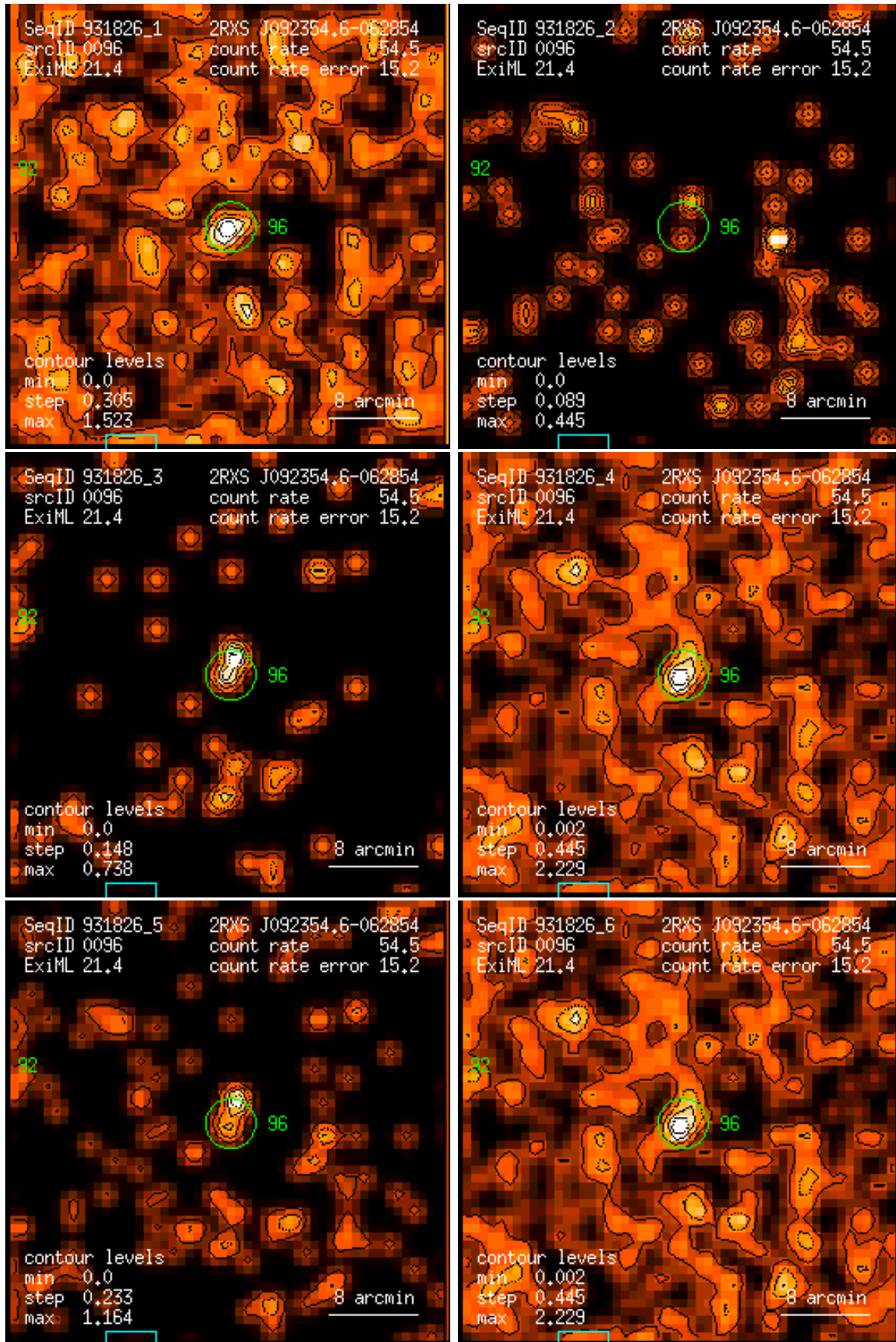
Figure 96: RASS 931826: detection 0096: band rate images, Gaussian filter: (1) PSPC channels 11 – 41, (2) 52 – 90, (3) 91 – 201, (4) 11 – 235, (5) 52 – 201, (6) 11 – 201. Broad band rates in counts/ks. Band rate contour levels in counts/ks/arcmin 2 .
