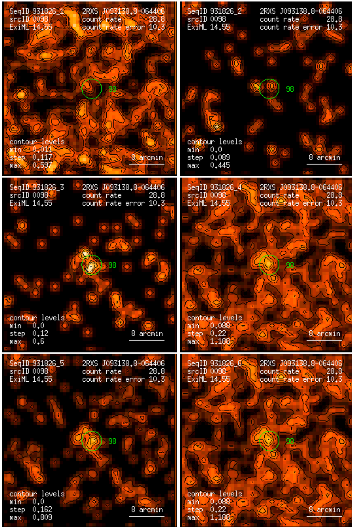
Figure 98: RASS 931826: detection 0098: band rate images, Gaussian filter: (1) PSPC channels 11 – 41, (2) 52 – 90, (3) 91 – 201, (4) 11 – 235, (5) 52 – 201, (6) 11 – 201. Broad band rates in counts/ks. Band rate contour levels in counts/ks/arcmin 2 .
