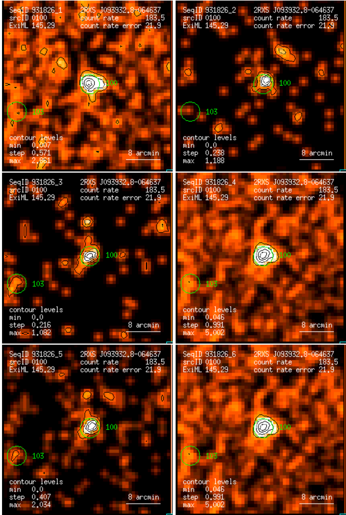
Figure 100: RASS 931826: detection 0100: band rate images, Gaussian filter: (1) PSPC channels 11 – 41, (2) 52 – 90, (3) 91 – 201, (4) 11 – 235, (5) 52 – 201, (6) 11 – 201. Broad band rates in counts/ks. Band rate contour levels in counts/ks/arcmin 2 .
