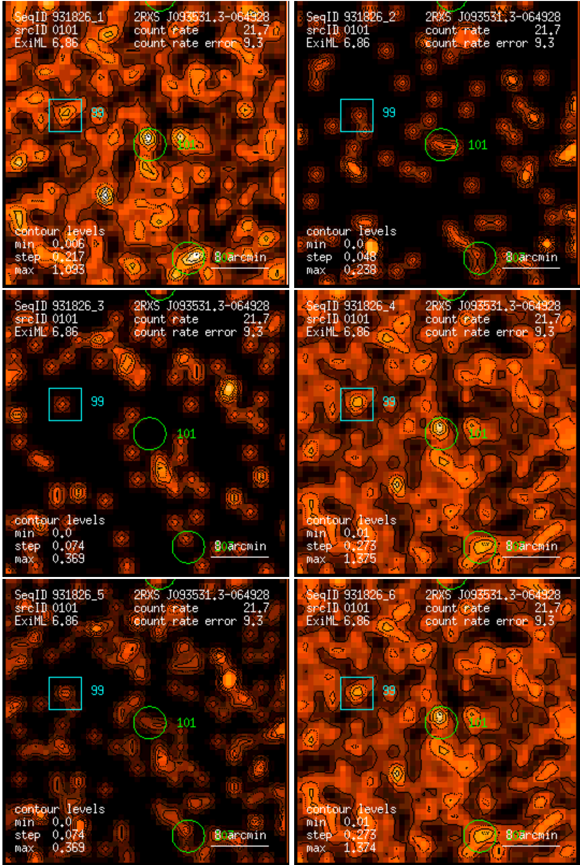
Figure 101: RASS 931826: detection 0101: band rate images, Gaussian filter: (1) PSPC channels 11 – 41, (2) 52 – 90, (3) 91 – 201, (4) 11 – 235, (5) 52 – 201, (6) 11 – 201. Broad band rates in counts/ks. Band rate contour levels in counts/ks/arcmin 2 .
