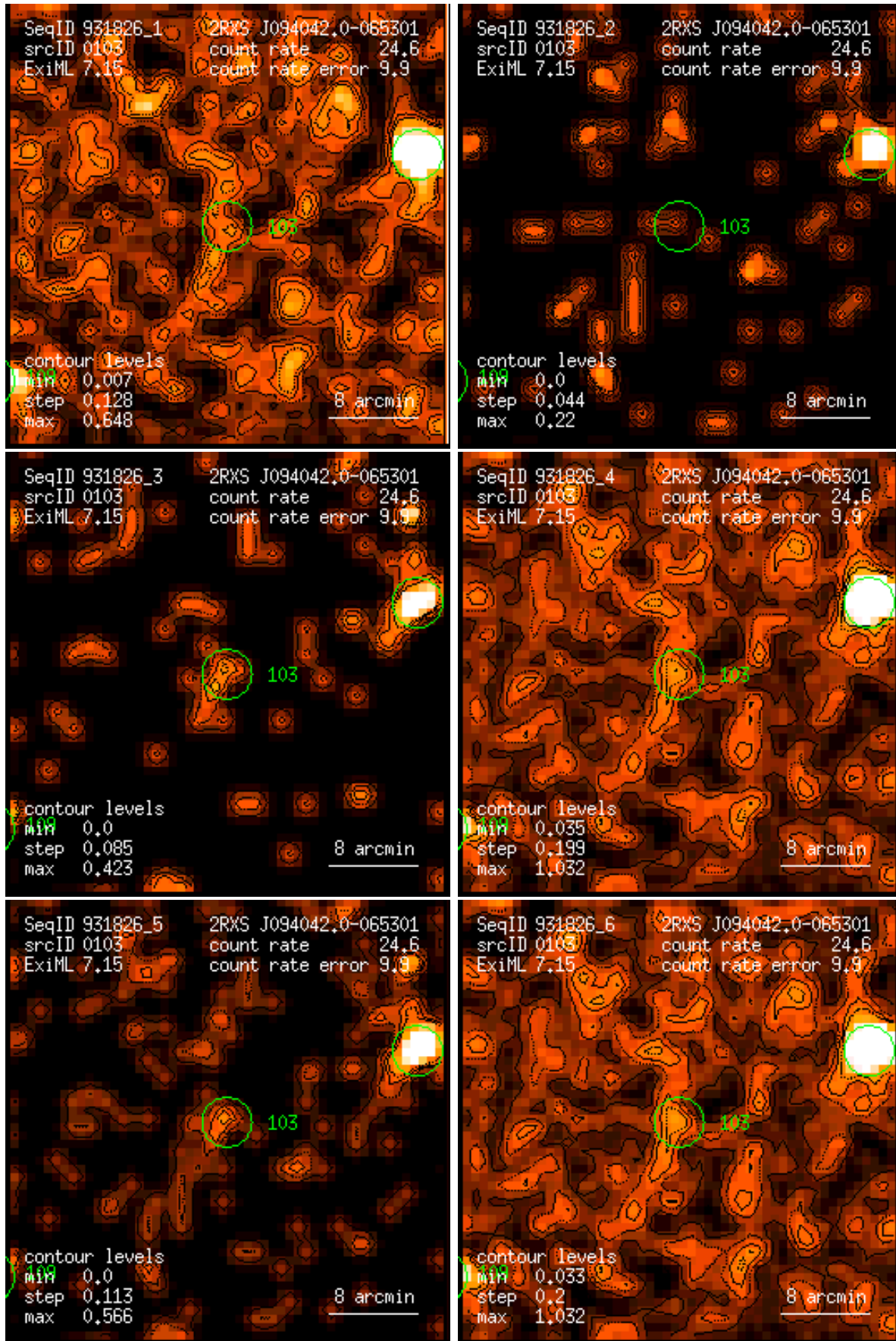
Figure 103: RASS 931826: detection 0103: band rate images, Gaussian filter: (1) PSPC channels 11 – 41, (2) 52 – 90, (3) 91 – 201, (4) 11 – 235, (5) 52 – 201, (6) 11 – 201. Broad band rates in counts/ks. Band rate contour levels in counts/ks/arcmin 2 .
