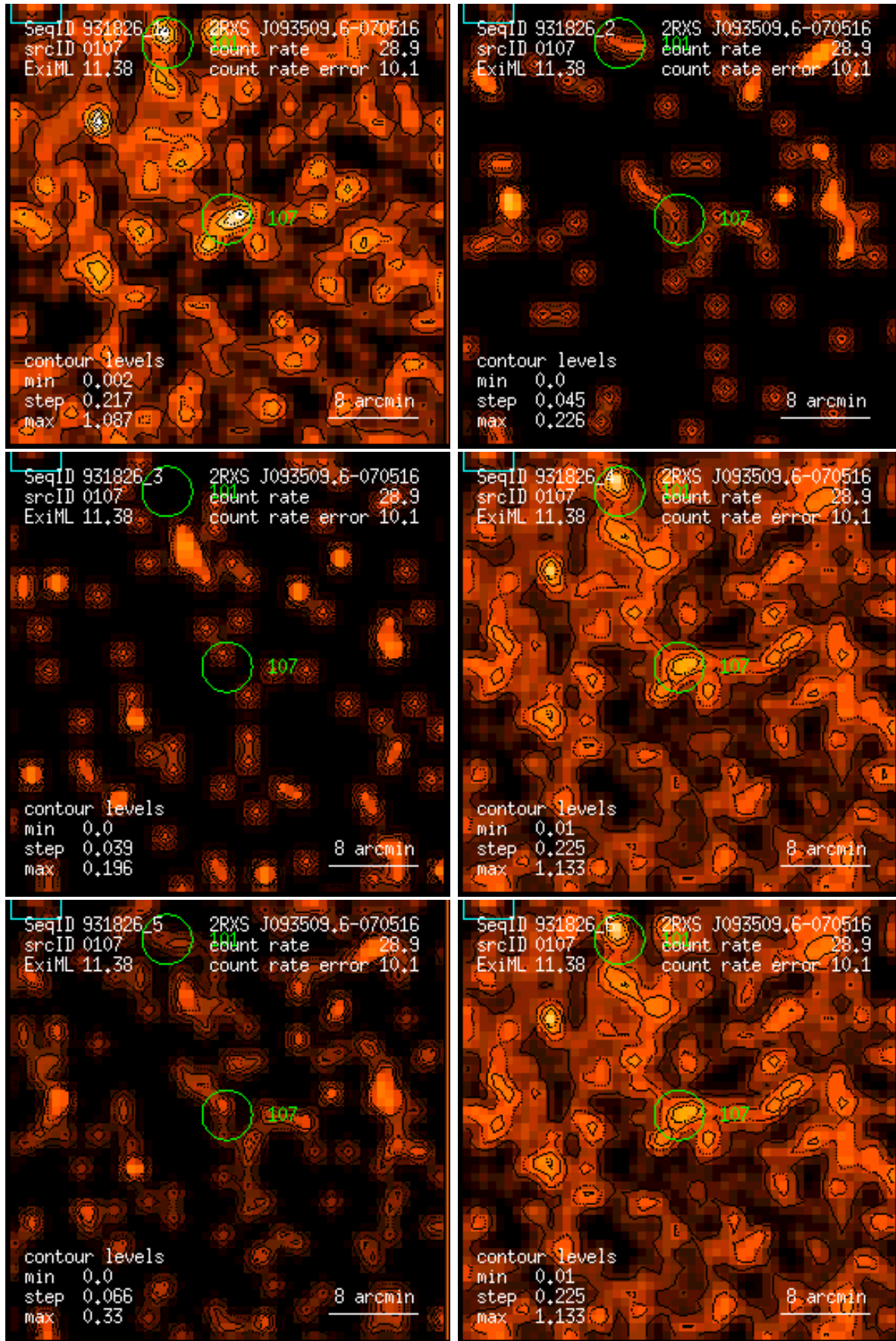
Figure 107: RASS 931826: detection 0107: band rate images, Gaussian filter: (1) PSPC channels 11 – 41, (2) 52 – 90, (3) 91 – 201, (4) 11 – 235, (5) 52 – 201, (6) 11 – 201. Broad band rates in counts/ks. Band rate contour levels in counts/ks/arcmin 2 .
