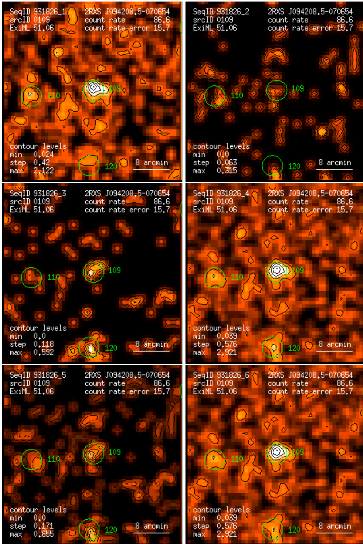
Figure 109: RASS 931826: detection 0109: band rate images, Gaussian filter: (1) PSPC channels 11 – 41, (2) 52 – 90, (3) 91 – 201, (4) 11 – 235, (5) 52 – 201, (6) 11 – 201. Broad band rates in counts/ks. Band rate contour levels in counts/ks/arcmin 2 .
