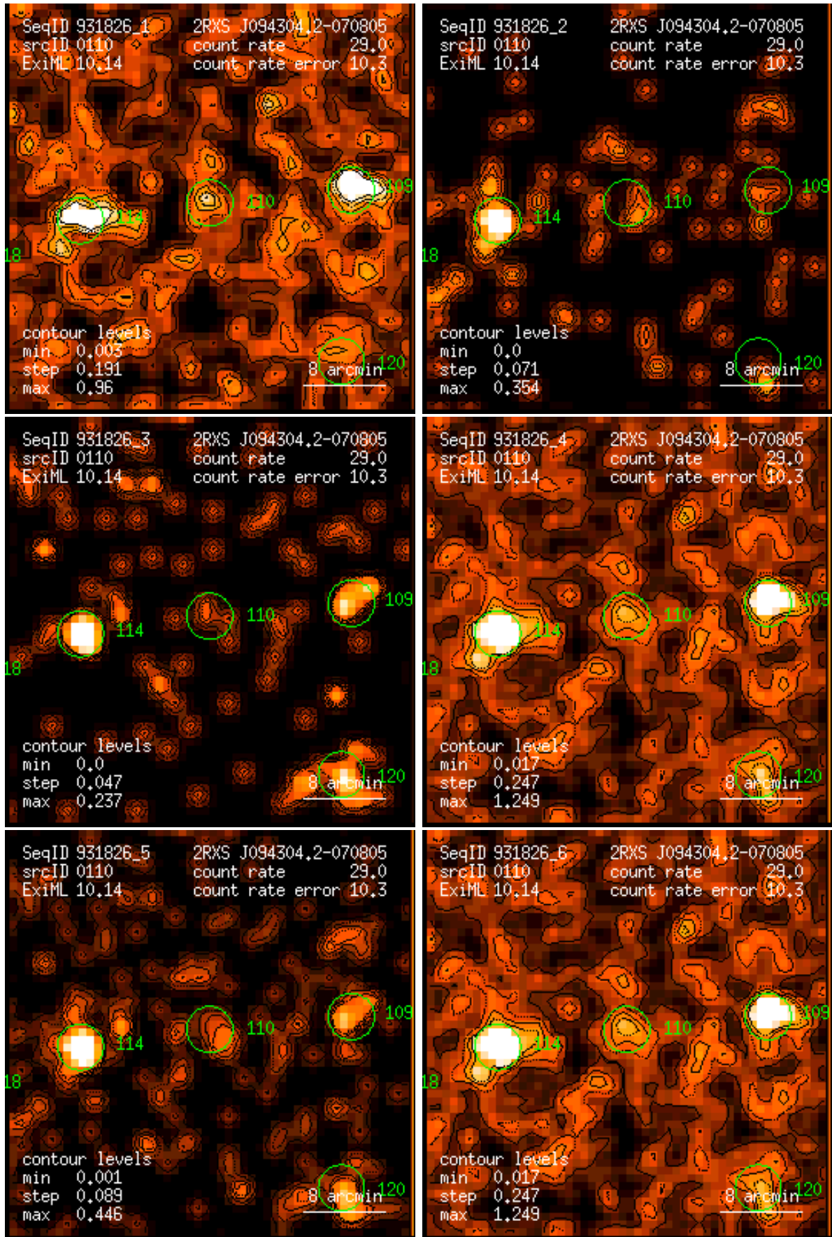
Figure 110: RASS 931826: detection 0110: band rate images, Gaussian filter: (1) PSPC channels 11 – 41, (2) 52 – 90, (3) 91 – 201, (4) 11 – 235, (5) 52 – 201, (6) 11 – 201. Broad band rates in counts/ks. Band rate contour levels in counts/ks/arcmin 2 .
