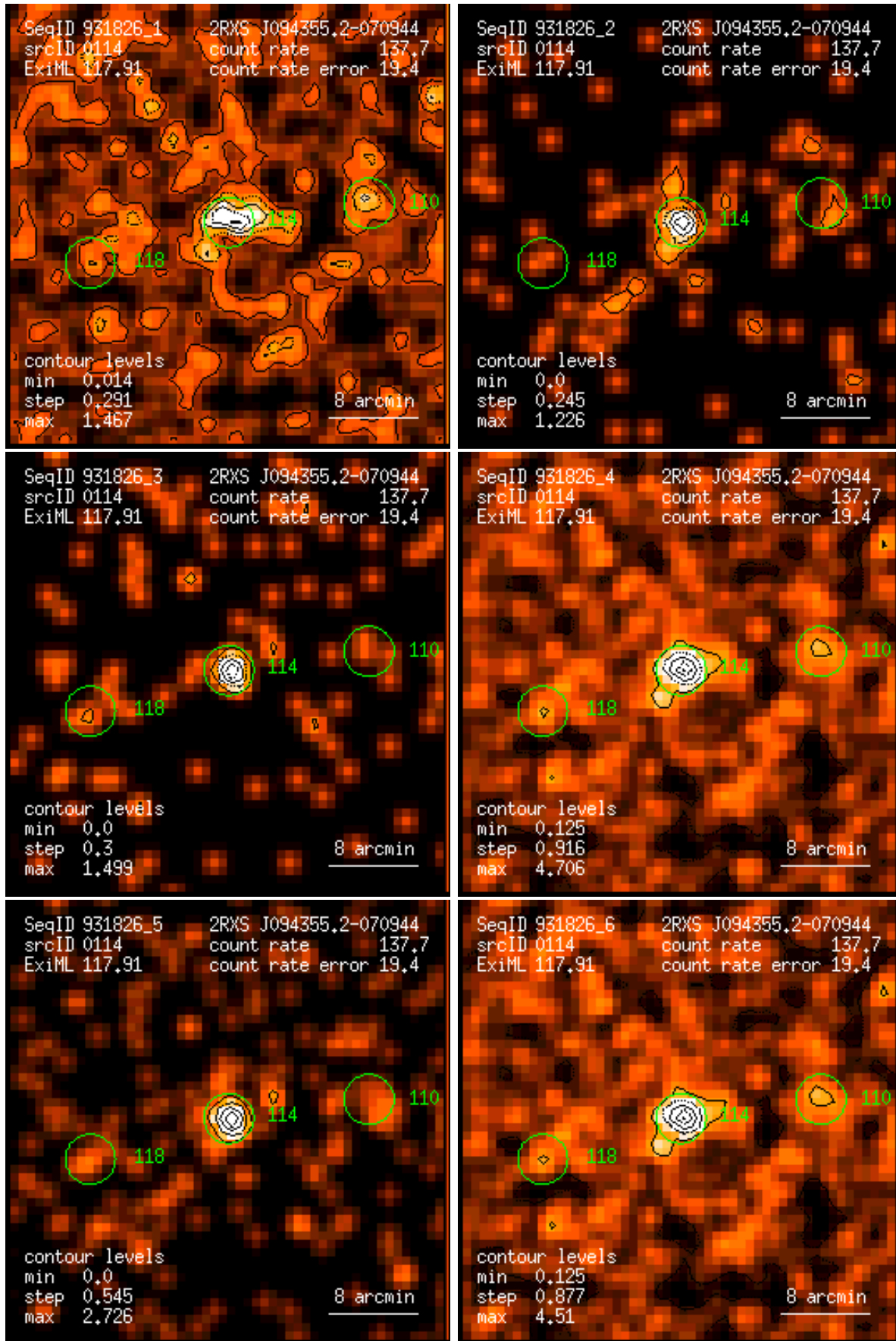
Figure 114: RASS 931826: detection 0114: band rate images, Gaussian filter: (1) PSPC channels 11 – 41, (2) 52 – 90, (3) 91 – 201, (4) 11 – 235, (5) 52 – 201, (6) 11 – 201. Broad band rates in counts/ks. Band rate contour levels in counts/ks/arcmin 2 .
