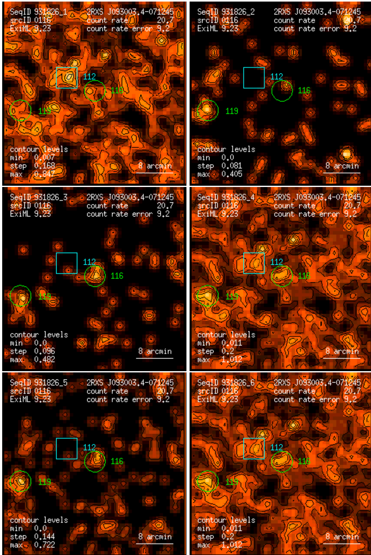
Figure 116: RASS 931826: detection 0116: band rate images, Gaussian filter: (1) PSPC channels 11 – 41, (2) 52 – 90, (3) 91 – 201, (4) 11 – 235, (5) 52 – 201, (6) 11 – 201. Broad band rates in counts/ks. Band rate contour levels in counts/ks/arcmin 2 .
